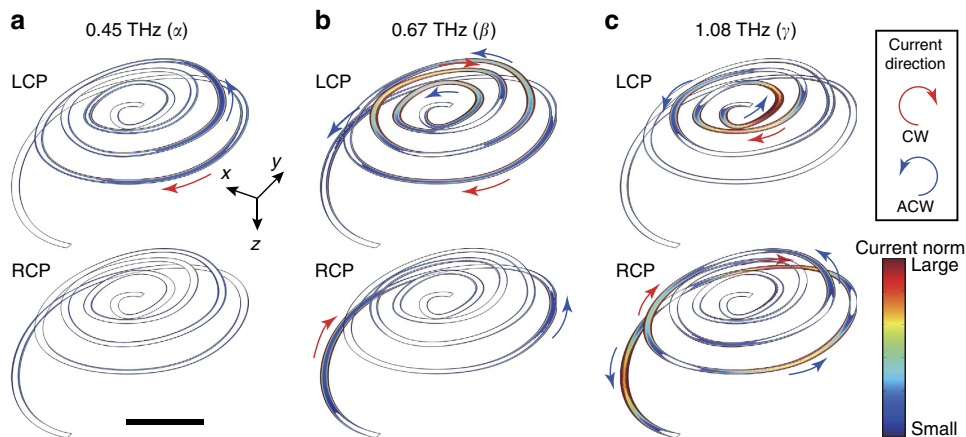
Figure 4 | Time-averaged current norm distributions on the 55- \mu m-height spiral for right and left circularly polarized light (denoted as RCP and LCP, respectively). (a–c) correspond to the distributions at the frequency of 0.45, 0.67 and 1.08 THz, respectively. The corresponding frequencies are indicated by markers in Fig. 3h as \alpha , \beta and \gamma , respectively. A bar in a indicates 50 \mu m. The arrows in these distribution figures indicate the current direction at a certain time: red and blue arrows correspond to the clockwise (CW) and anti-clockwise (ACW) current directions seen from the -z direction to +z direction.
