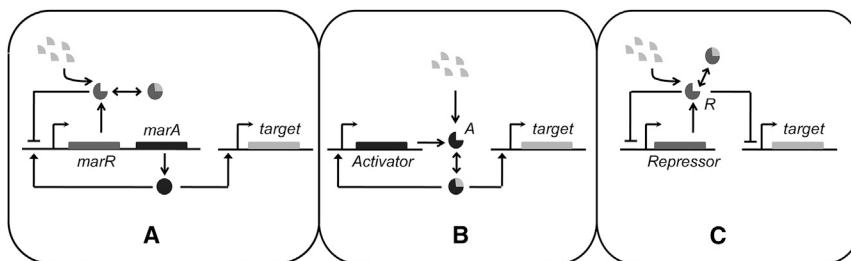
FIGURE 1 (A) Wild-type network design. MarR is an autorepressor (dark shaded). When bound to Inducer (light shaded), MarR is unable to control gene expression. MarA (solid) is an autoactivator. MarA also activates target gene expression. (B) Activator-only network design. Activator protein, A, is unable to control gene expression. When bound with inducer, A autoactivates and also activates target expression. (C) Repressor-only network design. Repressor protein, R represses its own and target expression. R bound with Inducer is unable to control gene expression.
