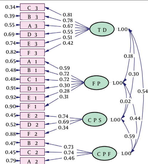
Figure 1. Confirmatory Factor Analysis (CFA) on 18 Items
