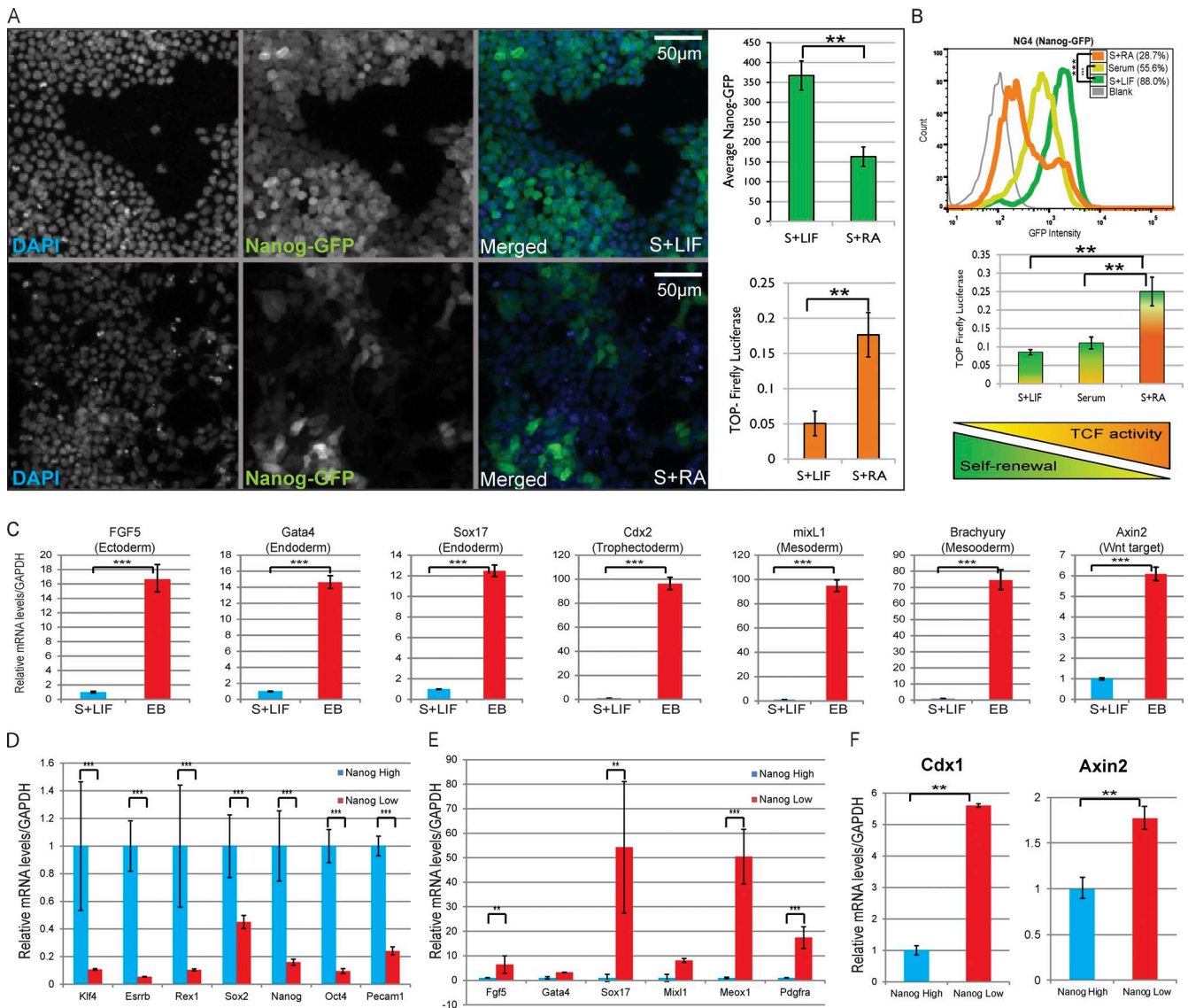
Figure 1. TCF-dependent transcriptional activation is up-regulated during mESC differentiation. (A) Mean Nanog-GFP levels (green bar graph; mean \pm SD of four replicates) in NG4-TOPFlash cells maintained in serum plus LIF (S+LIF; top) and serum plus RA (S+RA; bottom). Normalized TOPFlash reporter activity in simultaneously cultured NG4-TOPFlash (orange bar graph; mean \pm SD of three replicates). Resized original images shown are from a single representative experiment out of four replicates, with number of cells measured \geq 1,000 per experiment. (B) Comparison of Nanog-GFP (by flow cytometry, top; representative data of three replicates) and transfected TOPFlash (middle; mean \pm SD of three replicates) expression in mESCs cultured for 48 h in S+LIF, serum, or S+RA. Graphical summary reflecting inverse correlation between TCF-mediated transcriptional activity and self-renewal (bottom). (C) qPCR analysis of differentiation markers and TCF target genes in EBs versus the parental ESCs. Mean \pm SD of three replicates. (D) Relative mRNA levels of pluripotency markers in sorted Nanog High and Nanog Low mESCs. Mean \pm SD of two replicates. (E) Relative mRNA levels of differentiation markers in sorted Nanog High and Nanog Low mESCs. Mean \pm SD of two replicates. (F) Relative mRNA levels of TCF target genes Cdx1 (mean \pm SD of two replicates) and Axin2 (mean \pm SD of three replicates) in sorted Nanog High (S+LIF) and Nanog Low (S+RA) mESCs. **, P < 0.01 ; ***, P < 0.001 .
