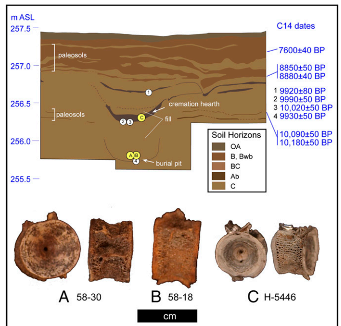
Fig. 2. Upward Sun River stratigraphy, chronology, and aDNA and stable isotope bone samples. Details provided in SI Text and Table S1.
