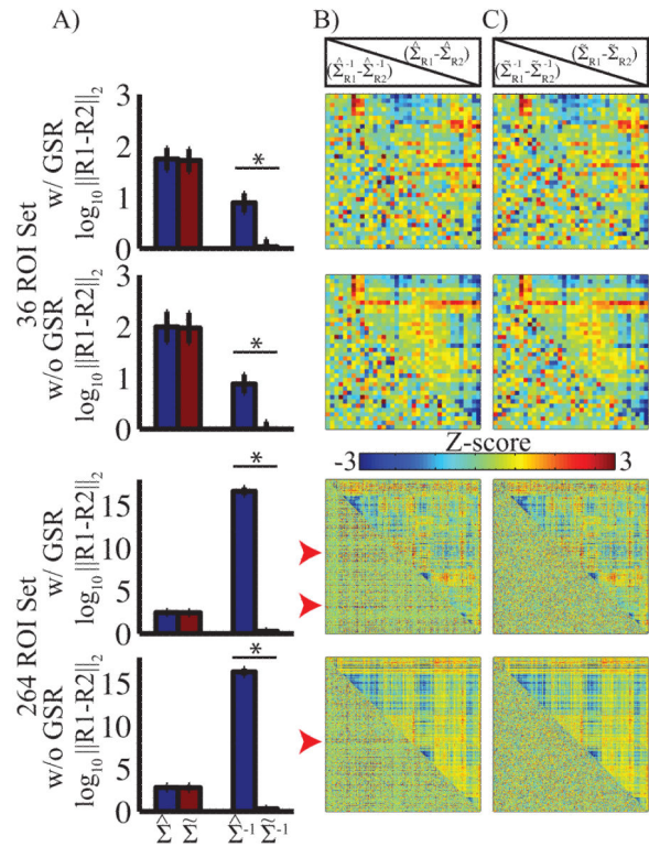
Figure 2. Matrix conditioning is sufficient to constrain the covariance inverse A: Mean Euclidean distance between covariance and inverse covariance matrices calculated from the first and second fMRI sessions. Blue bars display results without conditioning; red bars display results with conditioning. Error bars represent standard deviation across subjects. Asterisks indicate significant differences; in this case p < 0.001 . Conditioning had no significant effect on distance for full covariance results, but significantly reduced the distance (error) between the inverse covariance matrices. B: Z-transformed (removal of mean and normalization by standard deviation) mean difference between the first and second sessions without conditioning. Full covariance results are above the diagonal; partial covariance results are below the diagonal. Red arrow heads indicate organized pattern of large values in the inverse matrix. C: Same as B, but with conditioning. Structured noise is absent in the conditioned result.
