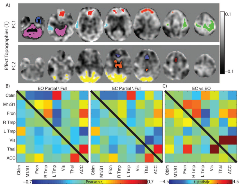
Figure 5. Partial Correlation Organization is Modulated by Brain-state
