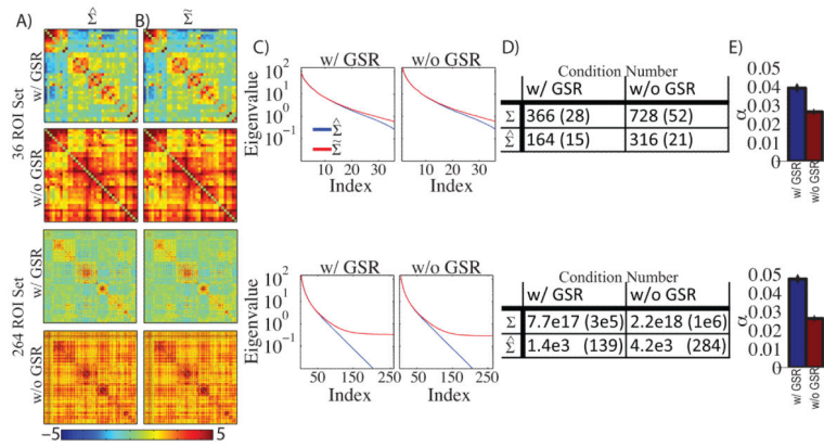
Figure 1. Matrix conditioning significantly improves the condition number of BOLD covariance matrices
