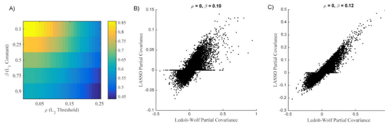
Figure 3. Ledoit-Wolf shrinkage and L 1 based methods yield similar results
