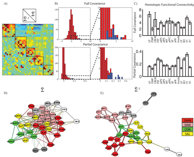
Figure 4. The partial covariance matrix is dominated by homotopic functional connectivity and contains RSN organization
