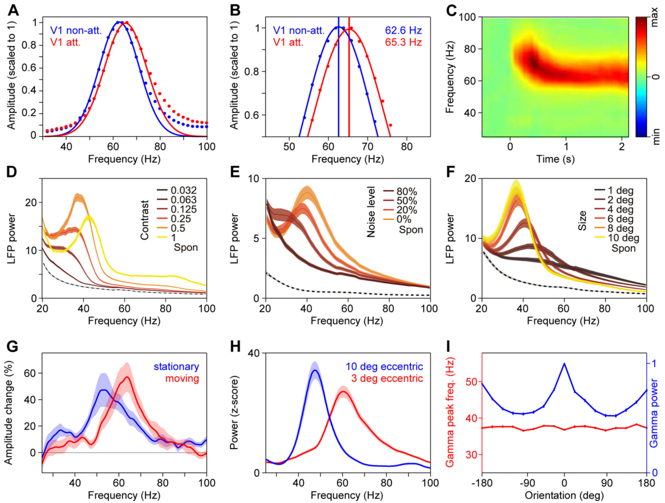
Figure 6. The gamma-band peak frequency increases with attention and salience
