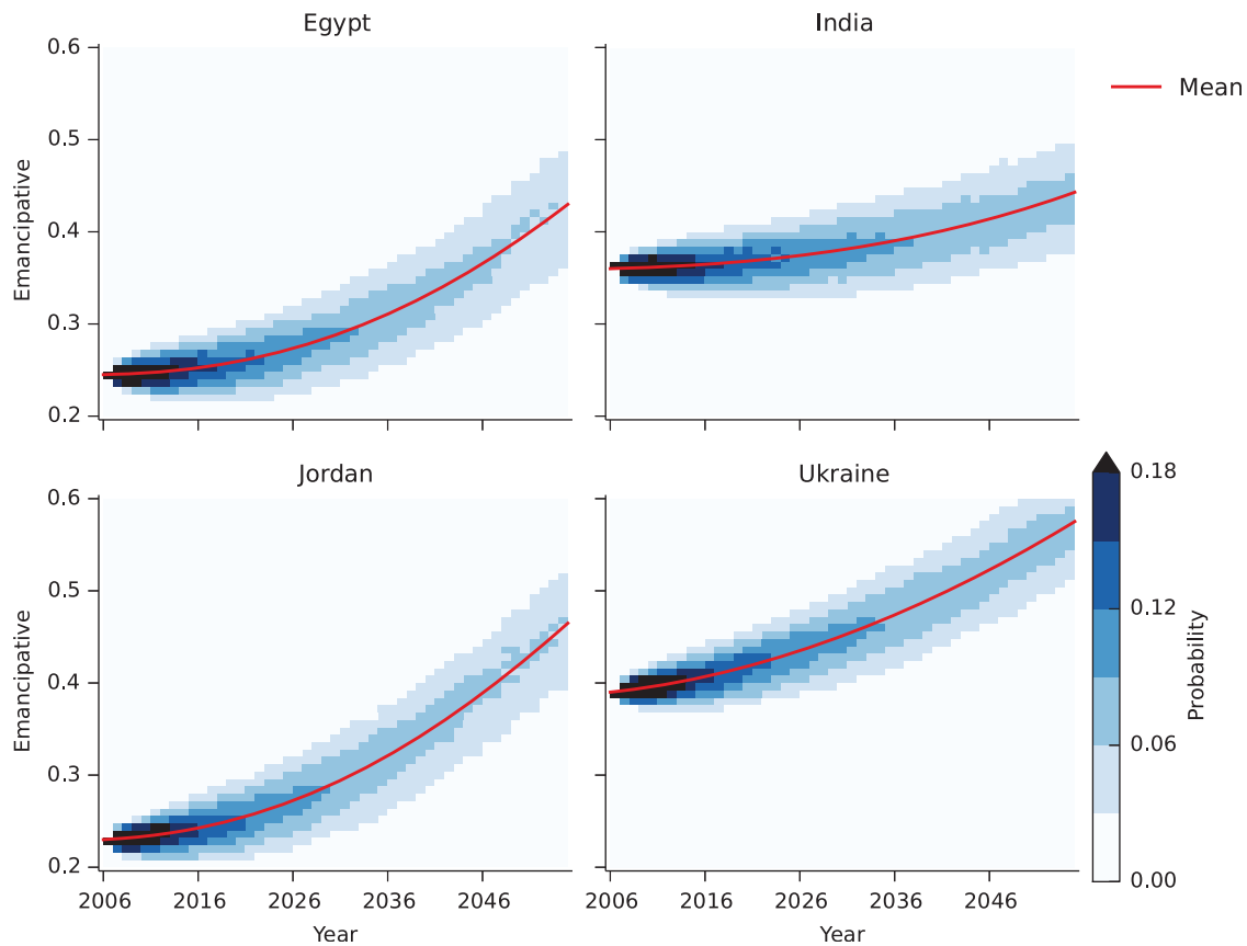
FIG. 6. Heatmaps showing the evolution of the distribution of E values in a set of 10,000 stochastic simulations of the model for Egypt, India, Jordan, and Ukraine. The starting time of the simulation for each country is 2006.
