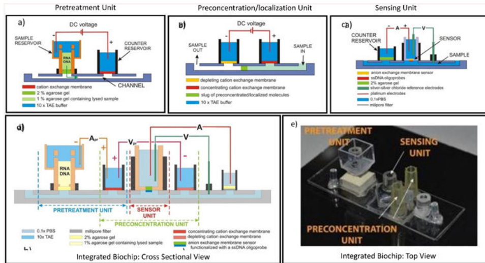
Figure 1. Schematics of a (a) pretreatment unit, (b) preconcentration unit (c) flow-through sensing unit, (d) integrated platform with all electrical connections. (e) Top view of an actual integrated device.
