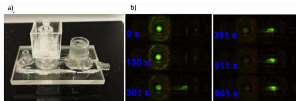
Figure 2. (a) Picture of the actual pretreatment unit. (b) Separation of a fluorescently labeled ssDNA from an oral cancer cell lysate,
