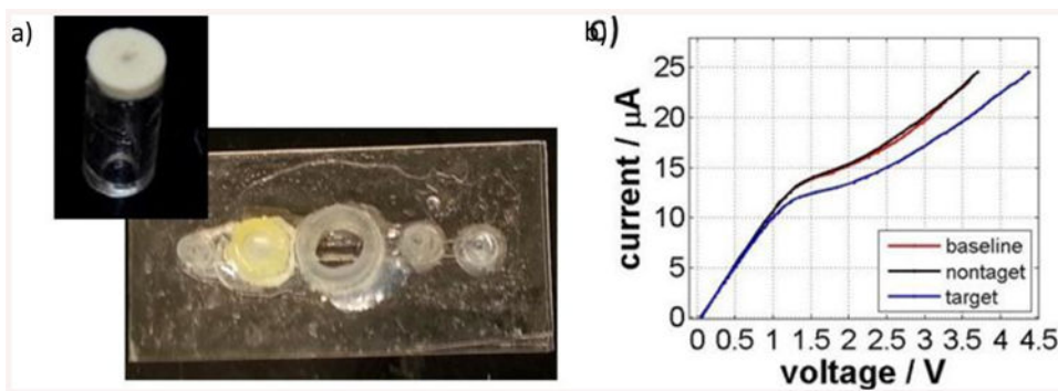
Figure 5. (a) Picture of an actual flow-through sensing unit and (b) Representative experiment showing specific detection of a DNA with a sequence corresponding to miRNA146a.
