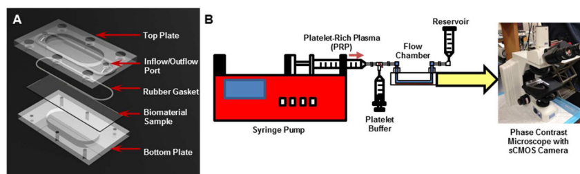
Figure 3. Parallel plate flow chamber system for platelet adhesion studies. (A) PRP was exposed to 10 \text{ dyne/cm}^2 for 5 min in a custom parallel plate flow chamber, with channel dimensions of 75 \times 25 \times 0.1 \text{ mm} . (B) The flow was controlled by a syringe pump with a 10 ml syringe that perfused PRP at 1.125 ml/min through the flow chamber into a reservoir. The flow was monitored via a 420 fps sCMOS camera mounted on a Nikon Eclipse ME600 microscope with 40X lens.
