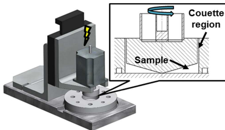
Figure 2. Shear exposure in the Hemodynamic Shearing Device (HSD). GFP suspended over the biomaterials were exposed to 1 \text{ dyne/cm}^2 and 20 \text{ dyne/cm}^2 for 12 min in the HSD, a computer-programmable cone-plate-Couette viscometer that exposes platelets to uniform shear stress and allows for real-time sampling.
