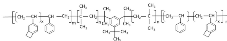
Figure 1. Schematic of poly(Styrene-coblock-4-vinylbenzocyclobutene)-polyIsoButylene-poly(Styrene-coblock-4-vinylbenzocyclobutene) (“xSIBS”).
