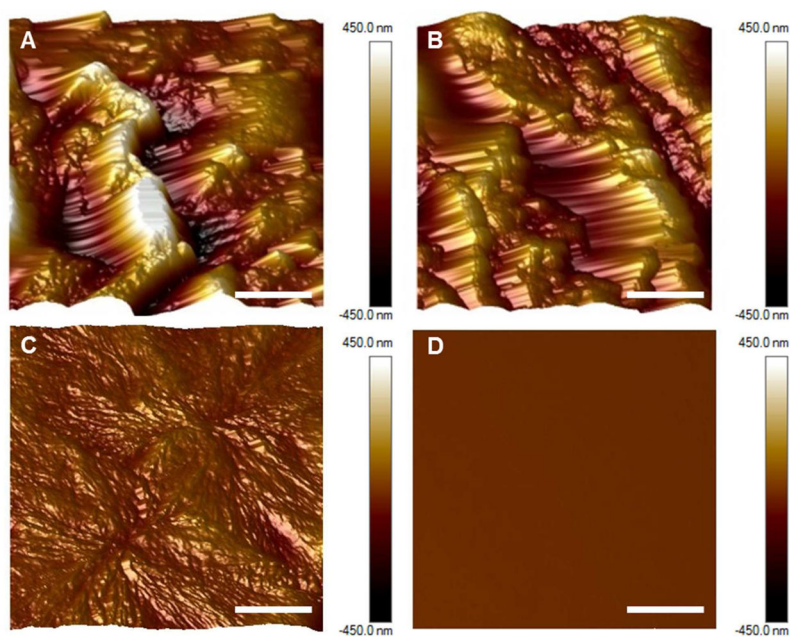
Figure 5. Surface analysis of xSIBS, PCL, and PMMA. AFM images taken of 20\ \mu\text{m} \times 20\ \mu\text{m} sections of (A) as-cast 25%-styrene xSIBs, (B) platelet-exposed 25%-styrene xSIBs, (C) PCL, and (D) PMMA ( 5\ \mu\text{m} lateral scale bar). Ordered styrene cylinder peaks with globular isobutylene valleys were observed on xSIBs. PMMA exhibited the lowest roughness.
