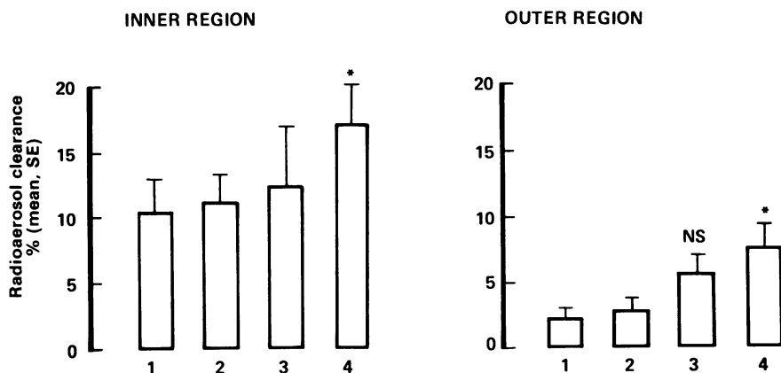
Fig 2 Mean (SE) regional clearance of radioaerosol during and after treatments 1-4 (see table). * p < 0.05 v treatment 2.
