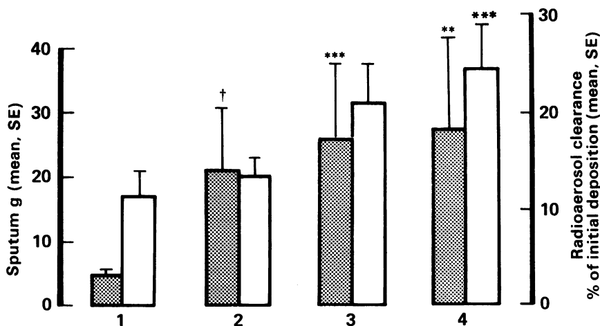
Fig 1 Mean (SE) sputum weight and whole lung radioaerosol clearance after treatments 1-4 (see table). Hatched columns indicate sputum and open columns radioaerosol. ** p < 0.02 and *** p < 0.01 v treatment 2; † p < 0.01 v treatment 1.
