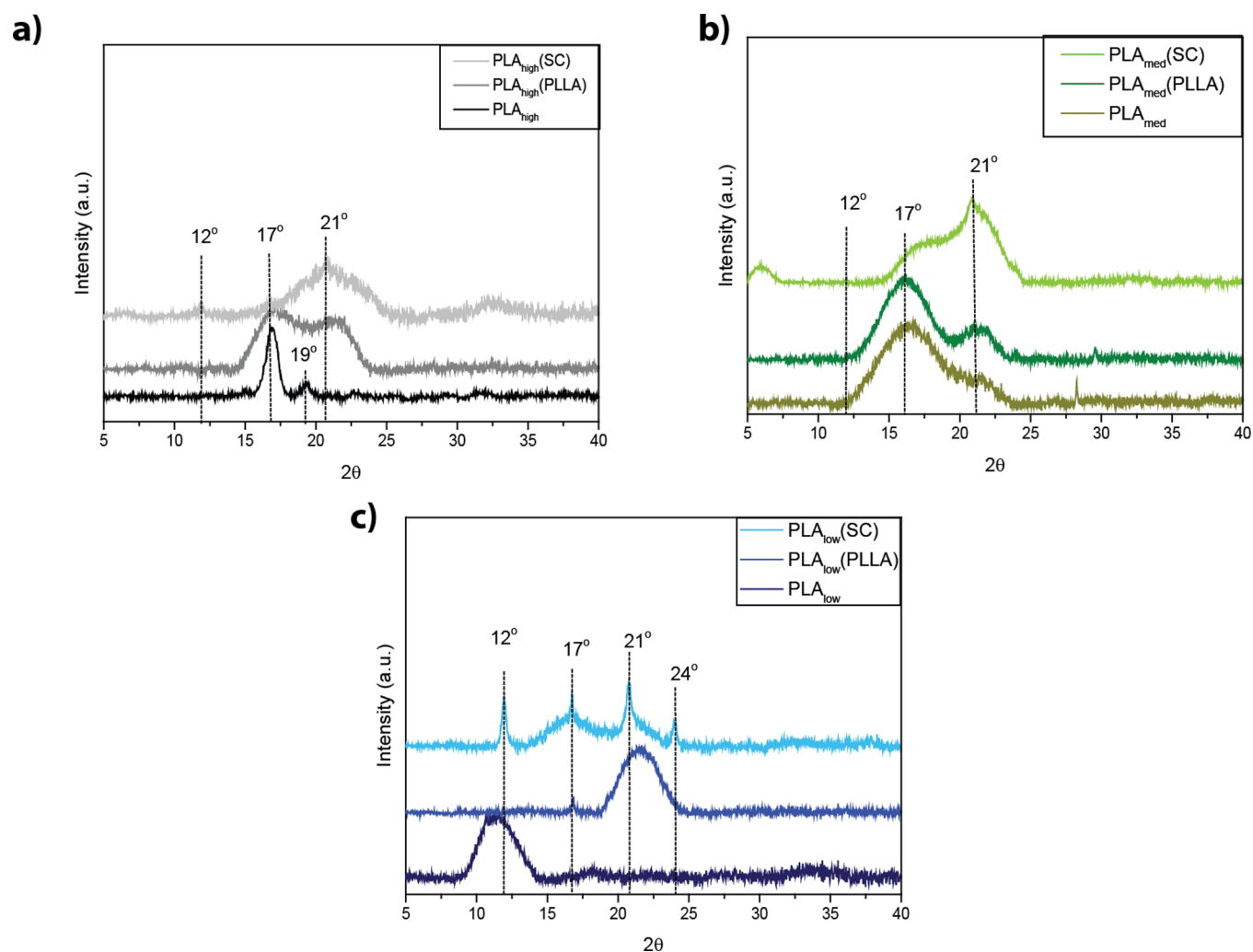
Figure 3. XRD patterns of the particulate-homocomposite materials: (a) PLA high -based, (b) PLA med -based and (c) PLA low -based homocomposites.
