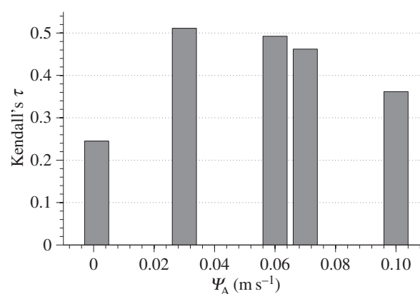
Figure 12. Kendall's \tau rank correlation coefficient calculated between in vivo and in silico \Delta\text{Th}/\text{Th} measurements obtained for the values of \Psi_A considered in this study. Simulations with an apposition threshold value of \Psi_A = 3 \times 10^{-2} \text{ m s}^{-1} obtained the strongest positive correlation ( p < 0.001 ).
