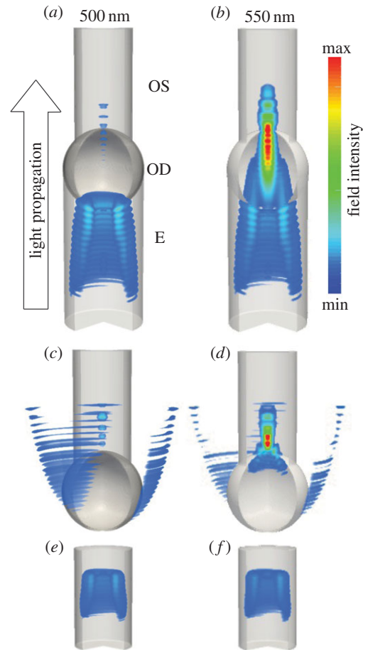
Figure 3. Simulated field intensity under monochromatic plane illumination within the ellipsoid (E), oil droplet (OD) and outer segment (OS) of the green single cone photoreceptor. The wavelength of illumination is 500 nm (a, c and e) 550 nm (b, d and f). Structures represent: full receptor model (a,b), no ellipsoid (c,d) and outer segment only (e,f).
