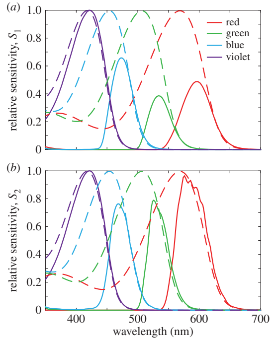
Figure 5. Relative sensitivities of the single cone photoreceptors calculated using two contrasting methods. (a) Relative sensitivities (solid lines) accounting for optical effects as shown in figure 4a, visual pigment absorbance template (dashed lines) and ocular media transmittance (equation (2.7)). (b) Relative sensitivities (solid lines) calculated by conventional methods using oil droplet transmittance, ocular media transmittance and visual pigment absorbance template (dashed lines) (equation (2.8)). Relative sensitivity curves are normalized to the maximum in the violet cone in each case.
