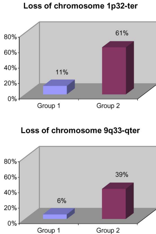
Fig. 3. Frequencies of sub-chromosomal imbalances in metastatic (group 2) and non-metastatic (group 1) colorectal cancers.
