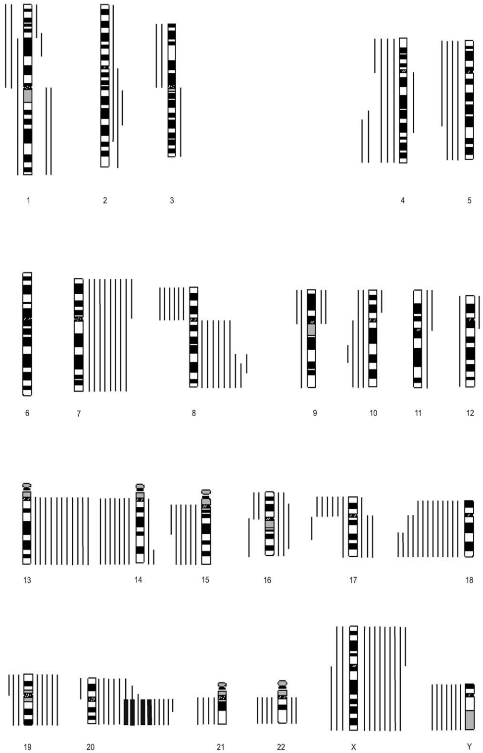
Fig. 1. Karyogram of chromosomal gains and losses in 18 colorectal carcinomas without liver metastases (group 1).
