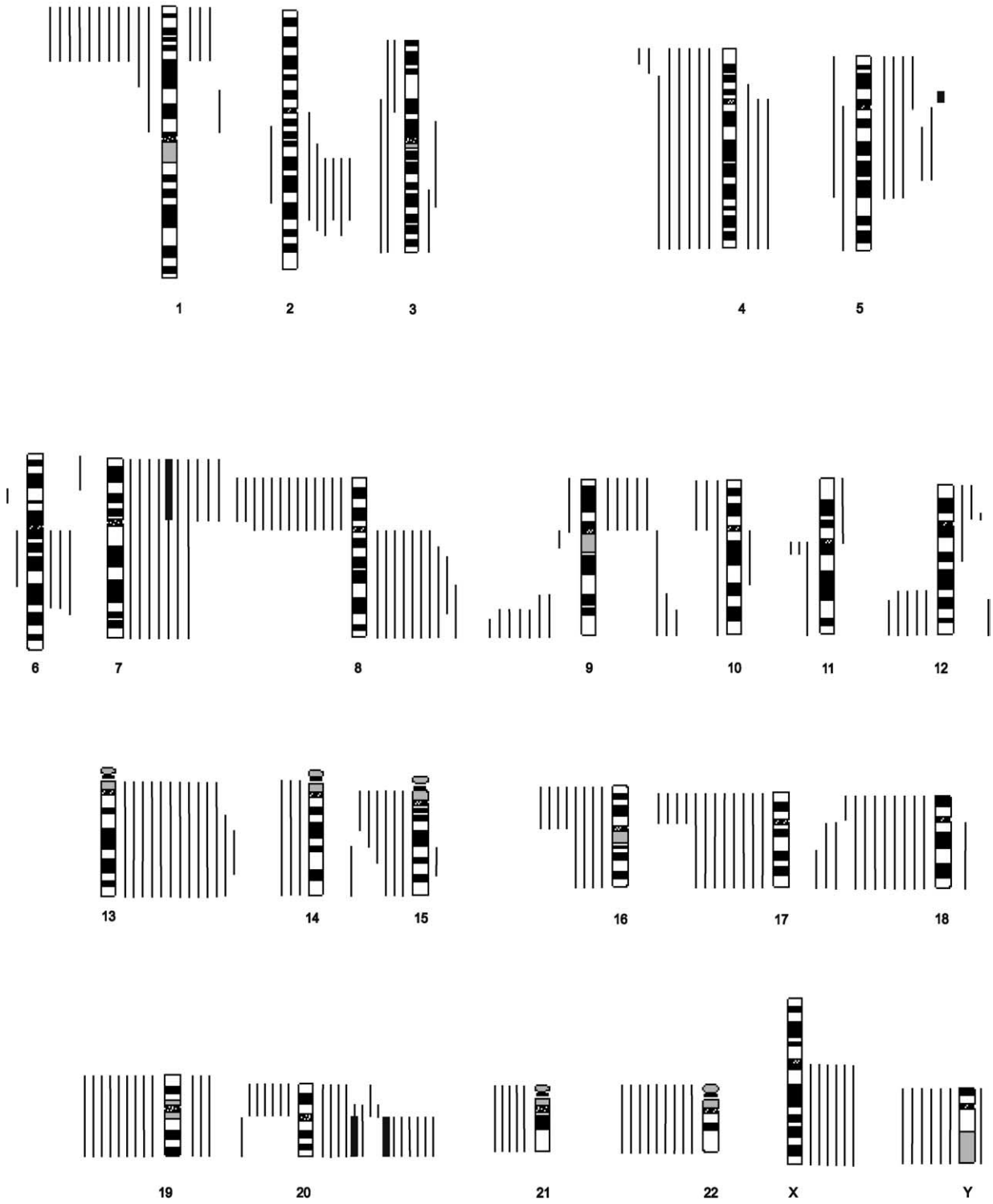
Fig. 2. Karyogram of chromosomal gains and losses in 18 colorectal carcinomas with synchronous liver metastases (group 2).
