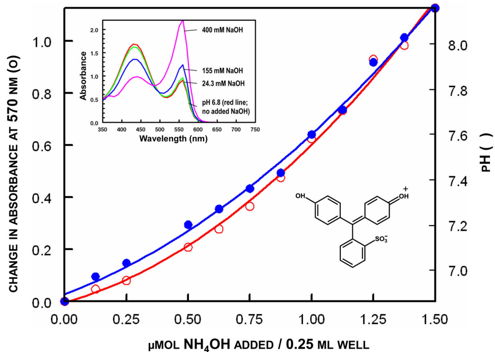
Figure 1. Microtiter well calibration curve for measurement of ammonia by change in absorption of phenol red. Aliquots of \text{NH}_4\text{OH} were added to 200 \mu\text{L} of 100 mM potassium phosphate, pH 6.8, containing 0.002% phenol red, and the changes in absorbance at 570 nm (O) and the pH (●) determined. The insets show the absorption spectra of phenol red upon addition of increasing quantities of NaOH, and the structure of the chromophore.
