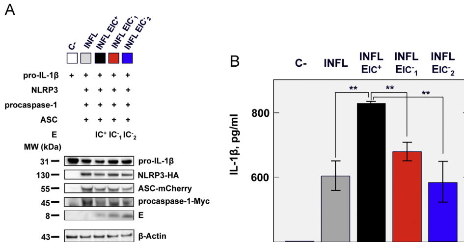
Fig. 5. Inflammasome activation through SARS-CoV E protein ion channel activity. The components of the NLRP3 inflammasome (INFL), NLRP3 (NLRP3-HA), ASC (ASC-mCherry), procaspase-1 (pro-caspase-1-Myc) and pro-IL-1 \beta were transfected in Vero E6 cells, in the absence or presence of SARS-CoV E protein with (IC + ) or without (IC - ) ion channel activity. EIC 1 - represents the N15A mutant and EIC 2 - indicates the V25F mutant. As a negative control, cells were transfected solely with pro-IL-1 \beta (C - ). (A) Western blot showing the presence of the inflammasome complex components and E protein within Vero E6 cells lysates. \beta -Actin was also detected as a loading control. (B) Levels of active IL-1 \beta present in the cell supernatant. Error bars represent standard deviations from three independent experiments. Statistically significant data are indicated with two asterisks (Student's t -test p value < 0.01).
