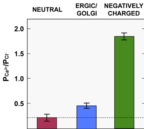
Fig. 2. \text{Ca}^{2+} selectivity of SARS-CoV E protein channel. Permeability ratios P_{\text{Ca}^{2+}}/P_{\text{Cl}^-} in neutral DPhPC (magenta column), ERGIC/Golgi (blue column) or negatively-charged DPhPS membranes (green column). Dotted line represents the permeability ratio value for a hypothetical neutral pore. Values above the line represent cation selectivity, and those below correspond to anion selectivity. Error bars show standard deviations.
