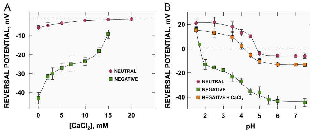
Fig. 3. Modulation of SARS-CoV E protein channel selectivity by \text{Ca}^{2+} . (A) Reversal potential (Erev) was measured in asymmetric (500 mM | 50 mM) KCl solutions upon addition of millimolar \text{CaCl}_2 concentrations. Two series of experiments were performed: in neutral DPhPC (magenta circles) and negatively charged DPhPS membranes (green squares). Dotted line shows Erev value corresponding to a non-selective ion channel. (B) Effect of pH on E protein Erev measured under the same KCl conditions above mentioned in neutral (magenta circles) and negatively charged membranes in the absence (green squares) or the presence of 15 mM \text{CaCl}_2 (orange squares). Dotted line shows the Erev value corresponding to a non-selective ion channel. Error bars represent standard deviations from three independent experiments.
