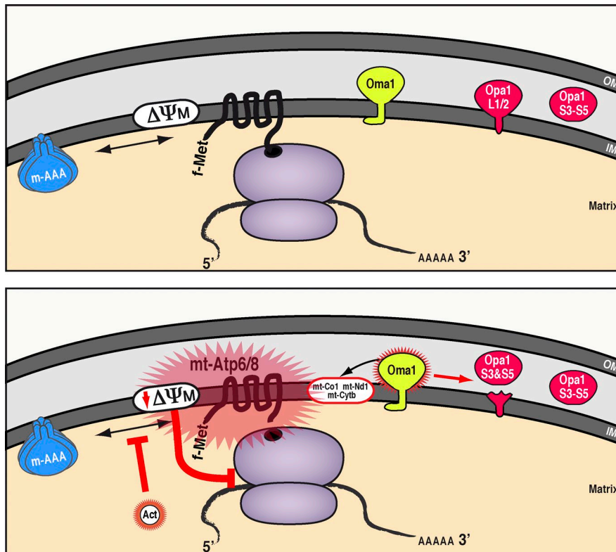
Figure 10. Model for quality control of mitochondrial protein synthesis and the mechanism for actinonin inhibition. (top) Wild-type scenario in mitochondria: the m-AAA protease ensures de novo proteins synthesized on mito-ribosomes do not overaccumulate in the inner membrane. (bottom) Impairing the turnover of de novo mitochondrial proteins either by actinonin treatment or the loss of m-AAA leads to polypeptide overaccumulation in the inner membrane, in particular the two subunits of the ATP synthase, mt-Atp6 and mt-Atp8. The membrane stress can dissipate the mitochondrial membrane potential, which in turn activates the metalloprotease Oma1 that processes the long Opa1 isoforms required for inner membrane fusion and modulates the abundance of selected de novo mitochondrial proteins. Prolonged disruptions to the mitochondrial inner membrane feed back onto mitochondrial translation elongation by stalling mito-ribosomes and preventing further protein synthesis. IM, inner membrane; \Delta\Psi_M , mitochondrial membrane potential; OM, outer membrane.
