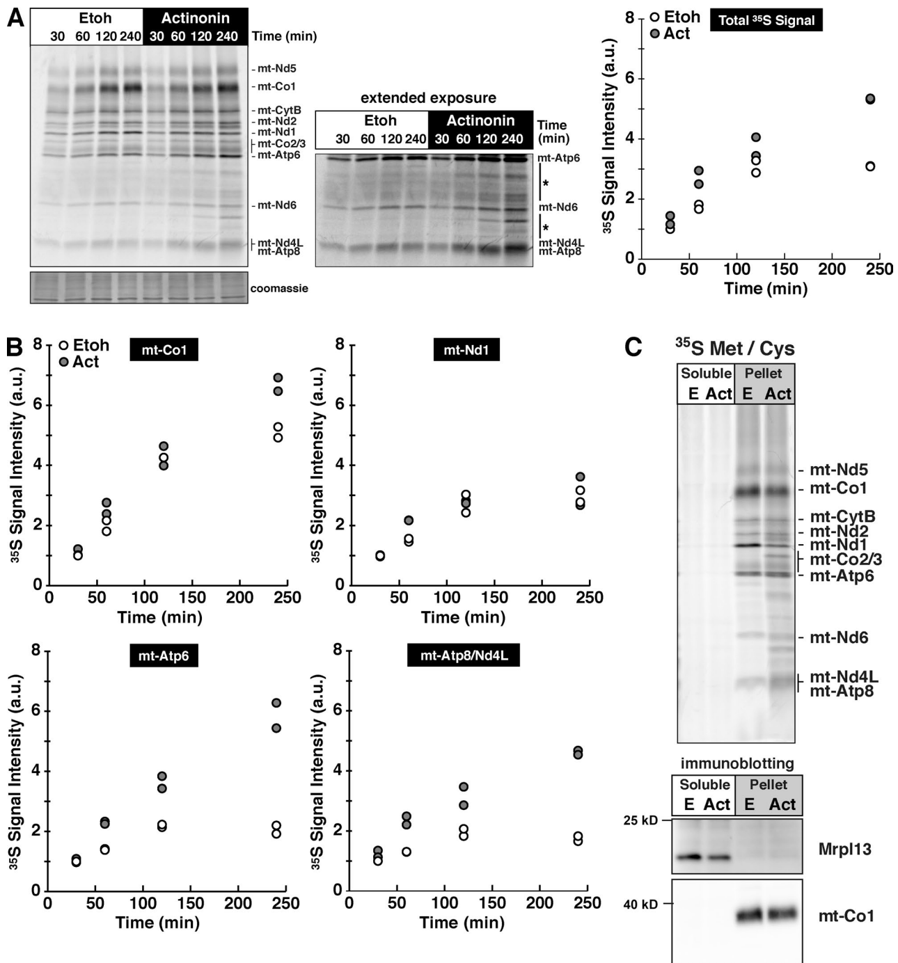
Figure 1. Actinonin induces a time-dependent aberrant accumulation of mitochondrial polypeptides in the inner membrane. (A, left) Pulse 35 S metabolic labeling with ethanol (Etoh) or actinonin (Act) in MEFs for the indicated time points. The asterisks indicate the accumulation of novel translation products. (right) Signal quantification determined for all translation products relative to the signal intensity at 30 min in the control from two independent experiments. (B) Quantification of 35 S signal intensity with time of selected mitochondrial polypeptides. (C, top) Sodium carbonate extraction of 35 S-labeled mitochondrial translation products. (bottom) Immunoblotting for membrane-anchored mt-Co1 and ribosomal protein Mrp13. a.u., arbitrary units.
