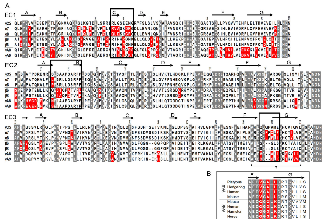
Figure 4. Candidate specificity determining residues
