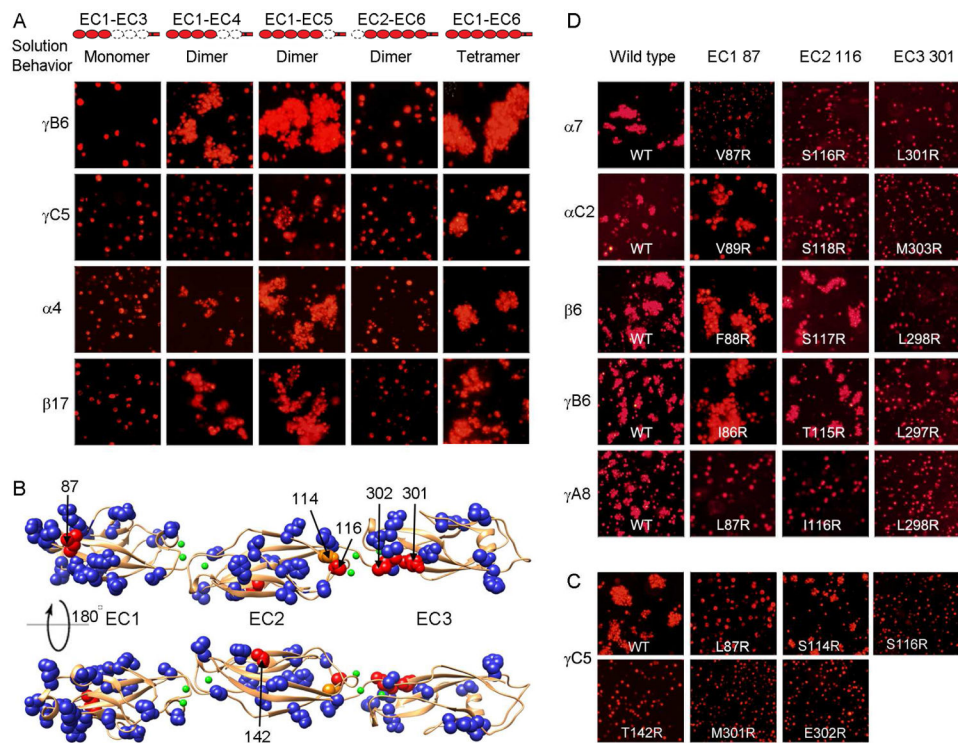
Figure 2. Elements of Pcdh cis and trans binding
