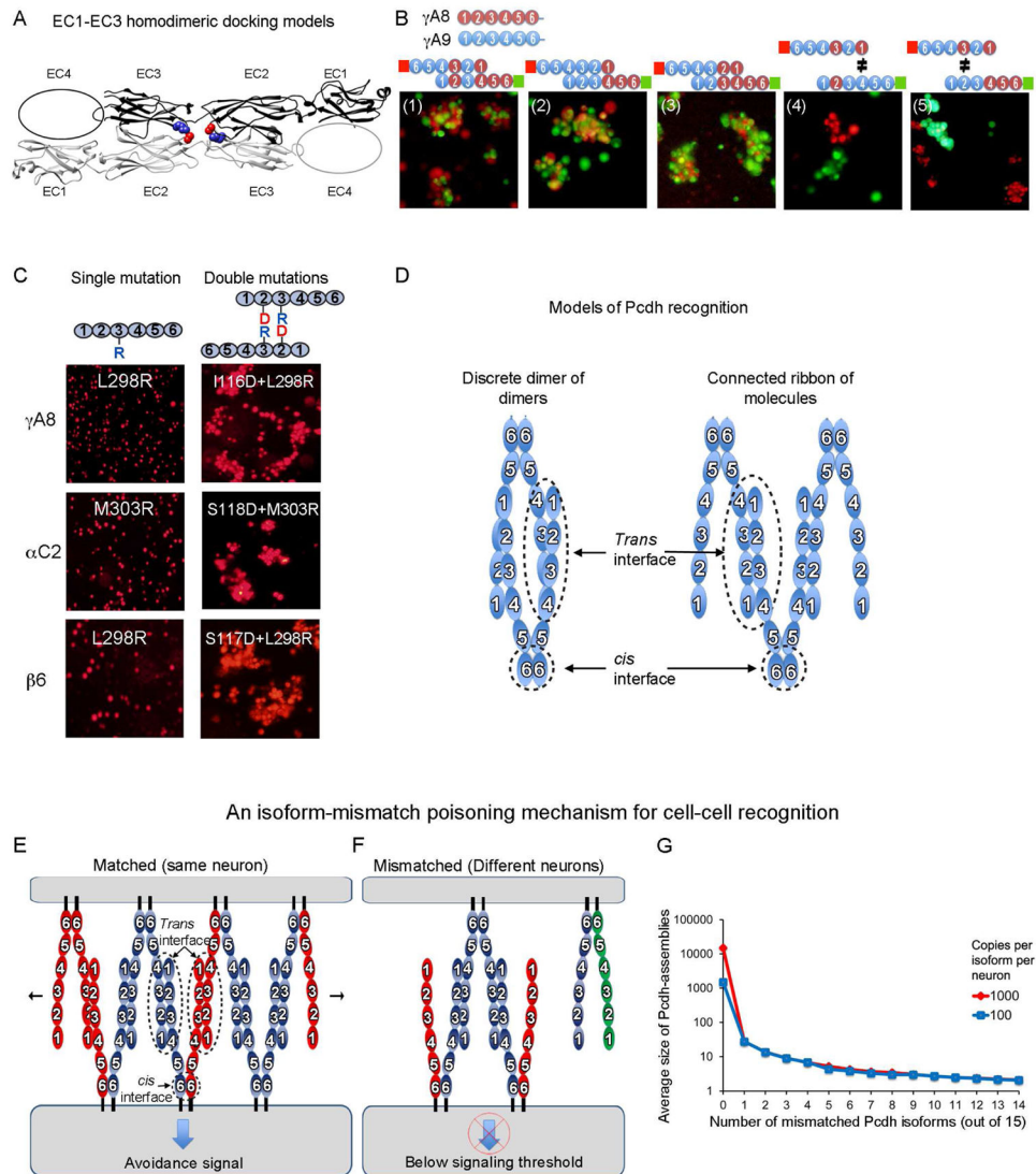
Figure 6. Molecular logic of Pcdh-mediated cell-cell recognition
