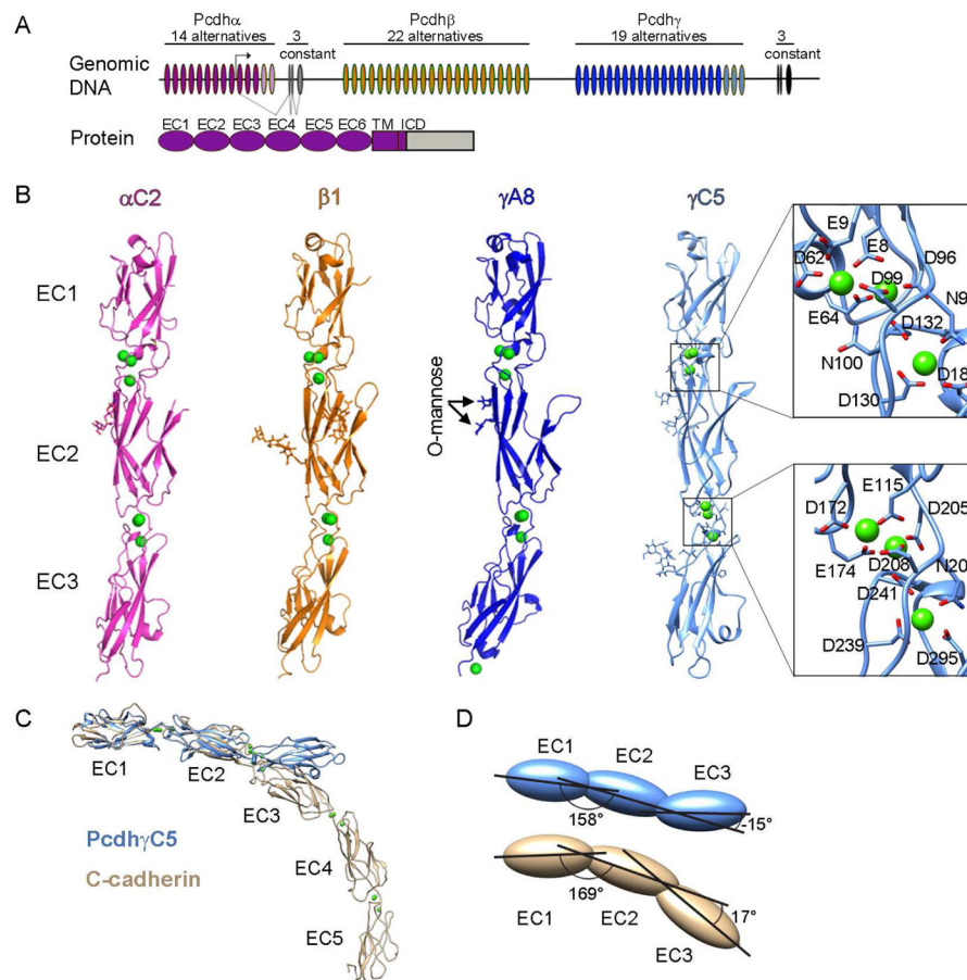
Figure 1. Crystal structures of four Pcdh EC1-EC3 isoforms
