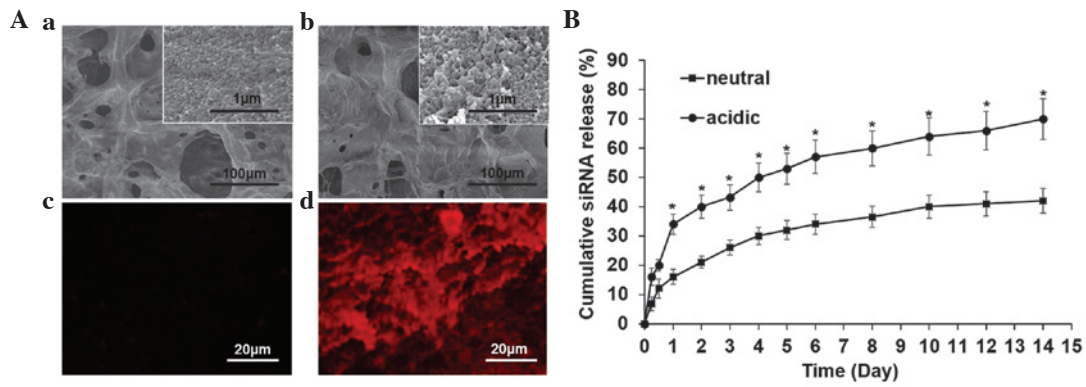
Figure 2. Surface observation of the (Aa) siRNA-free gel and the (Ab) gel loaded with siRNA using scanning electron microscope and (Ac and d) fluorescence microscope, respectively. (B) Cumulative siRNA release profile under neutral and acidic conditions, determined using the RiboGreen assay. Data are expressed as the mean \pm standard deviation. * P < 0.05 , compared with neutral. siRNA, small interfering RNA.
