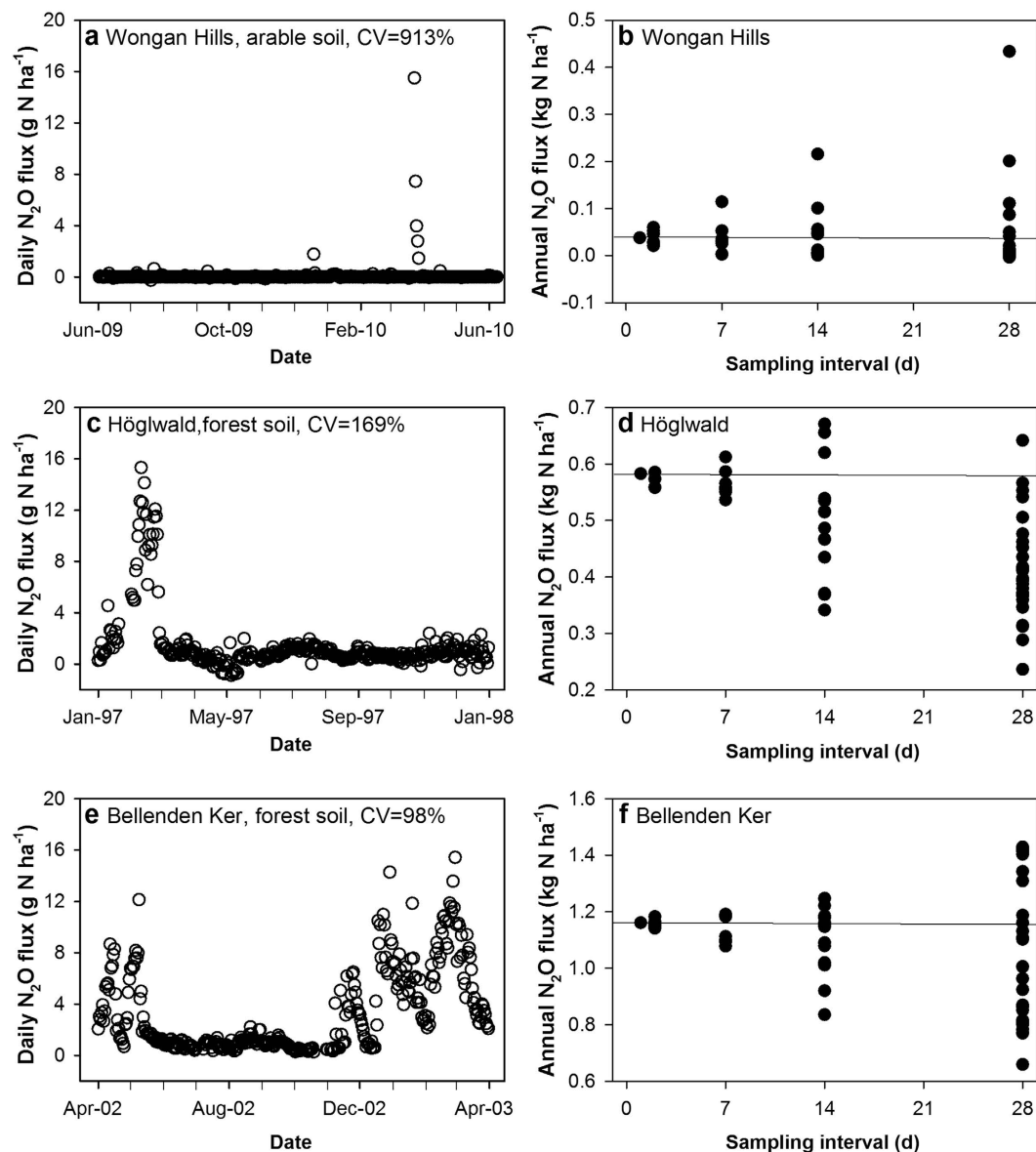
Figure 1. Daily N 2 O fluxes and the influence of sampling frequency on annual N 2 O fluxes. The daily N 2 O flux (a,c,e) for the three data sets shown have varying coefficients of variation (CV), which influences the effect of sampling frequency on annual N 2 O fluxes (b,d,f). See Table 4 for description of sampling intervals.
