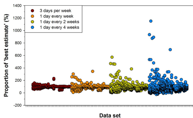
Figure 2. The proportion (%) of the ‘best estimate’ annual N 2 O flux estimated by each sampling frequency. For each dataset (28), the average annual flux estimate (calculated from replicate chambers) for each sampling frequency (and each permutation, Table 4) was compared to the ‘best estimate’ flux calculated from the average daily fluxes (expressed as a %). The ‘best estimate’ was calculated using all daily fluxes. For each sampling frequency, the datasets are presented in the same order (from left to right in the above Figure) as that listed in Supplementary Table 1. Specific values for each dataset are listed in Supplementary Table 1.
