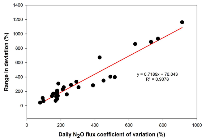
Figure 3. Relationship between the coefficient of variation of the daily N_2O flux and the deviation (range) from the ‘best estimate’ annual N_2O flux. For each dataset (28; represented as single point in the above Figure), the range in deviation was determined after comparing the annual N_2O fluxes calculated from a sample interval of 4-weekly (every 28 days) with the ‘best estimate’ for each permutation (Table 4). The ‘best estimate’ was calculated using all daily fluxes. Specific values for each dataset are listed in Supplementary Table 1.
