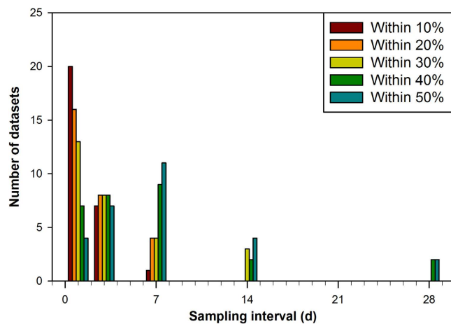
Figure 4. Impact of sampling interval on estimating annual N_2O fluxes at a given accuracy. The number of datasets obtaining annual N_2O fluxes at a given accuracy are listed as a function of sampling interval. Specific values for each datasets are listed in Supplementary Table 1.
