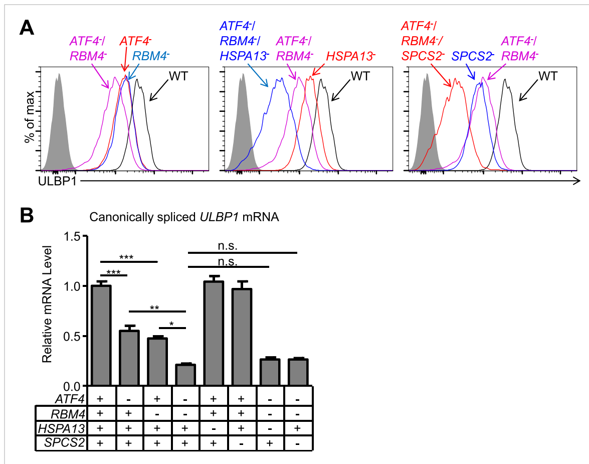
Figure 3. Double and triple-mutant cell lines show stepwise decreases in ULBP1 expression. (A) Flow cytometric analysis of ULBP1 expression on single, double, and triple-mutant HAP1 cells. ATF4 -/- /RBM4 -/- double-mutant cells were generated by mutagenesis of ATF4 in RBM4 -/- cells. Triple-mutant cells were generated by mutagenesis of HSPA13 or SPCS2 in ATF4 -/- /RBM4 -/- double-mutant cells. Shaded gray histograms represent isotype control staining. Data are representative of three independent experiments. (B) RT-qPCR analysis of canonically spliced ULBP1 mRNA expression levels in the cells described in (A) . Expression levels were normalized to ACTB, GAPDH, and HPRT1 and are shown as mean ±SE. The data were analyzed by 1-way ANOVA with Bonferroni's multiple comparisons test and substantive significant differences are shown. Data are representative of three independent experiments. *p < 0.05, **p < 0.01, ***p < 0.001, n.s.: not significant.
