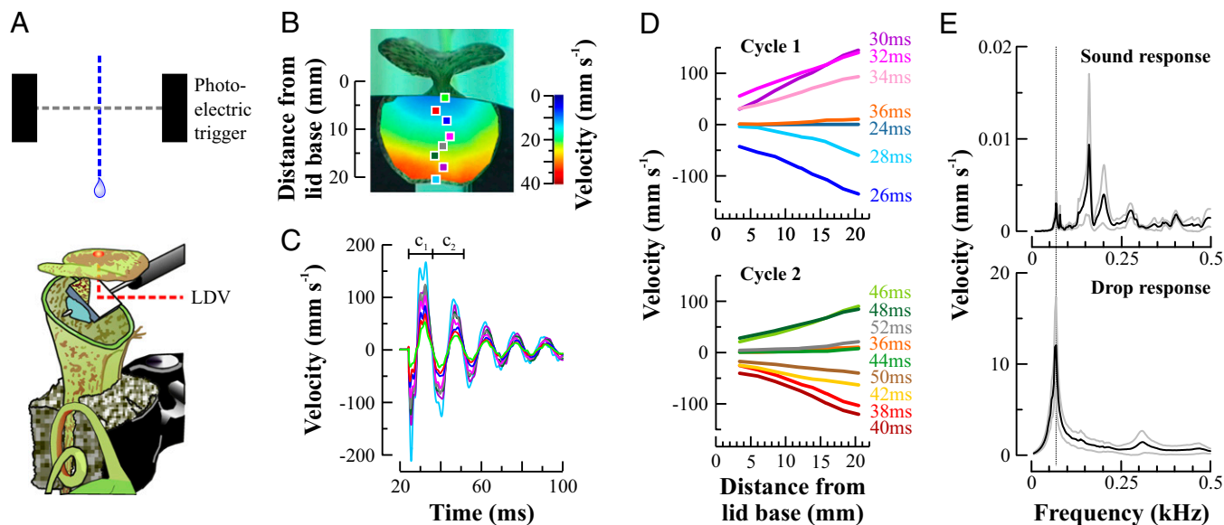
Fig. 3. High-resolution vibration analysis of an N. gracilis lid. (A) Experimental setup for measuring the drop impact response of the pitcher lid with a scanning laser Doppler vibrometer (LDV). A front coated mirror was used to deflect the laser beam onto the lower lid surface. (B) Velocity heat map of an impact response showing increasing velocity from lid base to tip. The colored squares highlight eight sample scan points along the centerline of the lid. (C) Time-resolved lid oscillation constructed from sample points in B ( c_1 and c_2 , cycles 1 and 2). (D) Deflection shapes of the N. gracilis lid during the first two oscillation cycles following drop impact, showing a linear increase of velocity along the length of the lid. The first cycle is characterized by shorter period and higher velocities than subsequent cycles (cf. C). (E) Frequency spectrum of the lid vibration in response to a 0.1- to 2-kHz sound sweep (Top) and a simulated rain drop impact (Bottom). The black lines represent the average response spectrum calculated for all measurement points, and the gray spectra represent the SD.
