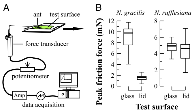
Fig. 4. Ant friction forces on pitcher lid surfaces. (A) Experimental setup. (B) Peak friction forces generated by Crematogaster ants on the lower lid surfaces of N. gracilis ( n = 3 ) and N. rafflesiana ( n = 2 ) pitchers in comparison with control surfaces (glass). Bars denote medians, boxes represent the inner two quartiles, and whiskers contain all values within 1.5 times interquartile range. For statistics see text.
