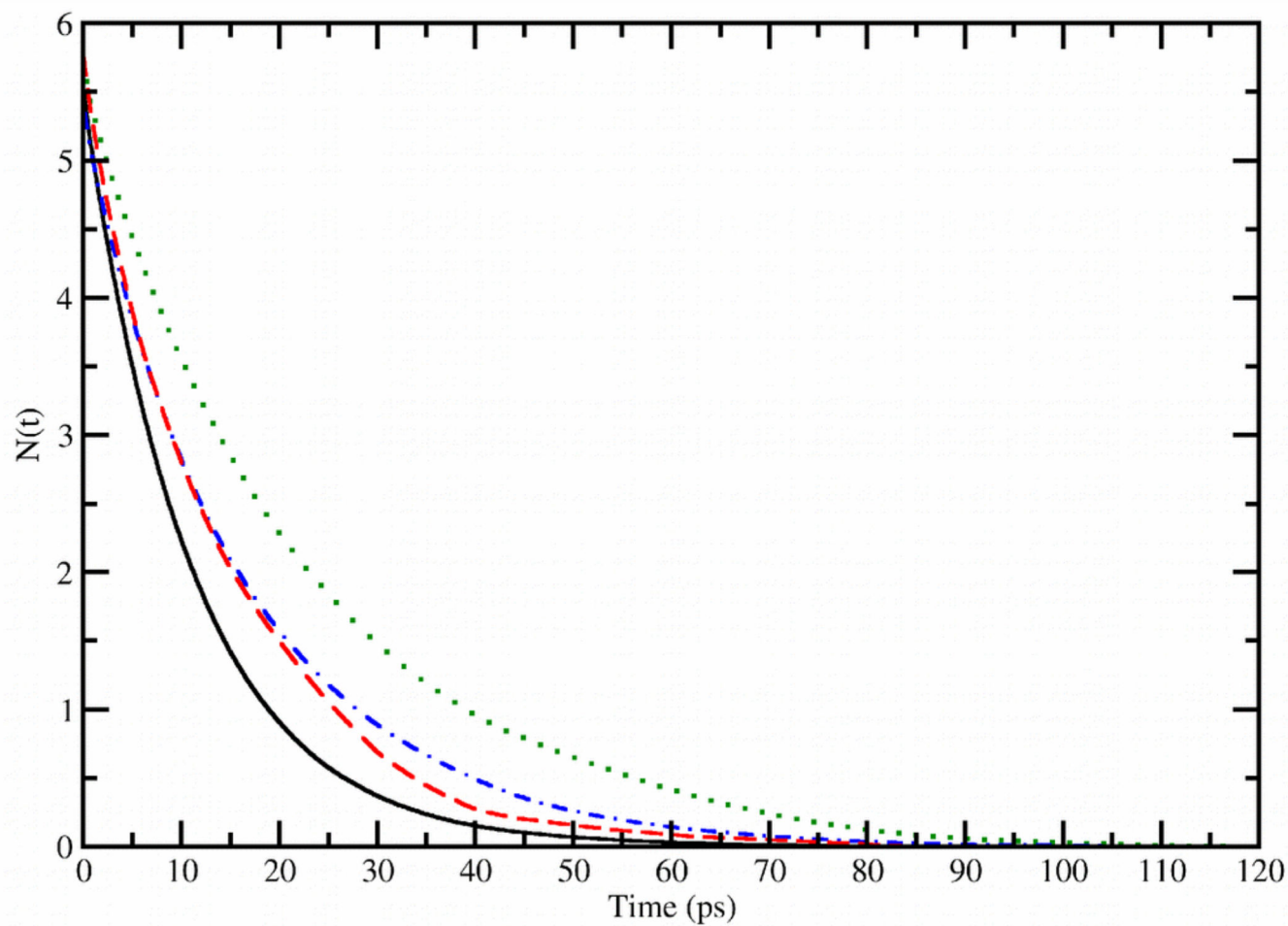
Figure 6. First shell residence time of water molecules obtained from the Na + simulations. The plot shows the results obtained using fixed charges with GROMOS96 parameters (black, Na1 ), fluctuating charges with GROMOS96 parameters (dashed red, Na2 ), fluctuating charges modifying only \sigma (dot-dashed blue, Na3 ) and fluctuating charges modifying both \sigma and \epsilon (dotted green, Na4 ).
