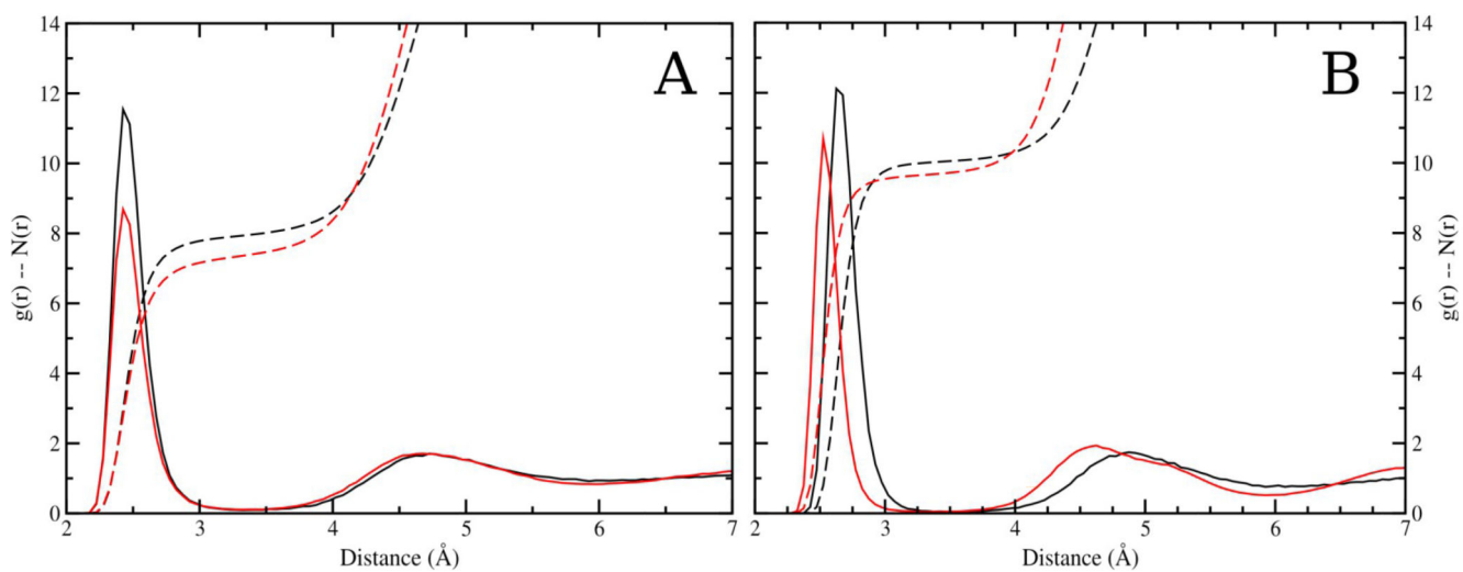
Figure 8. Comparison of ion-oxygen radial distribution functions (full lines) and relative integrals (dashed lines) obtained using either fixed charges (black) or fluctuating ones (red). Panel A: Ca^{2+} -O g(r) and N(r) ; Panel B: La^{3+} -O g(r) and N(r) .
