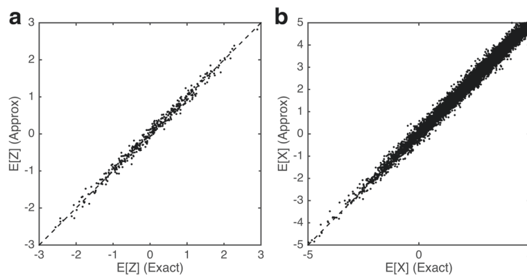
Fig. 2 Comparison of exact and block-based EM algorithms. Plots show the correlation between expectations computed using the exact and block-based EM algorithms for latent low-dimensional positions Z ( a ) and latent observations X ( b ). Simulations were performed on a simulated data set with 500 genes and 200 cells. A block size of 50 was chosen for the approximate approach
