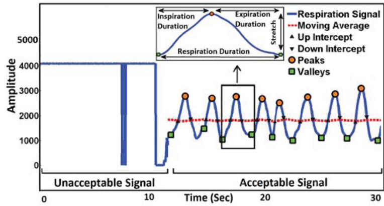
Figure 3. Illustration of acceptable/unacceptable RIP signals, and computation of base RIP features. The portion of signal that holds respiration signal property, looks like quasi-sinusoidal is marked as acceptable. Saturated at top is labeled unacceptable.
