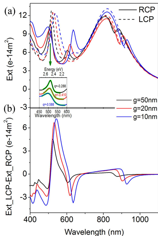
Figure 3. Optical activity with different gaps between the two nanorices. (a) Extinction spectra of the Au-Ag dimers ( l = 240 \text{ nm} , d = 60 \text{ nm} ) with g = 10 \text{ nm} (blue), 20 \text{ nm} (red) and 50 \text{ nm} (black) under LCP and RCP excitation. The inset shows the Fano fittings (green lines, I = A \frac{(q\gamma + \omega - \omega_0)^2}{(\omega - \omega_0)^2 + \gamma^2} + B ) of the indicated peaks for different gaps excited with RCP. The q values reflect the asymmetry of the peaks. (b) The CD spectra of the Au-Ag heterodimers with different gaps.
