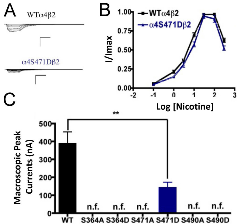
Fig. 2. Functional characterization of mutations on PKA putative sites in the \alpha4 subunit with nicotine used as agonist. (A) Family of nicotine-induced macroscopic currents for mutation \alpha4S471D\beta2 and the wild-type \alpha4\beta2 nAChR. Calibration bars are shown for all family of currents, horizontal bars indicate time (5 s) and vertical bars indicate the inward current (500 nA). (B) Dose-response relationships obtained by voltage-clamp using nicotine as agonist. Nicotine dose-response curves were determined using seven nicotine concentrations (0.1, 1, 3, 10, 30, 100 and 300 M). The responses were normalized to the maximum response ( I/I_{max} ). (C) Comparison of the nicotine-induced macroscopic peak currents of the mutations and wild-type receptor shown in nA ( n=6-17 ) (** p<0.005 ).
