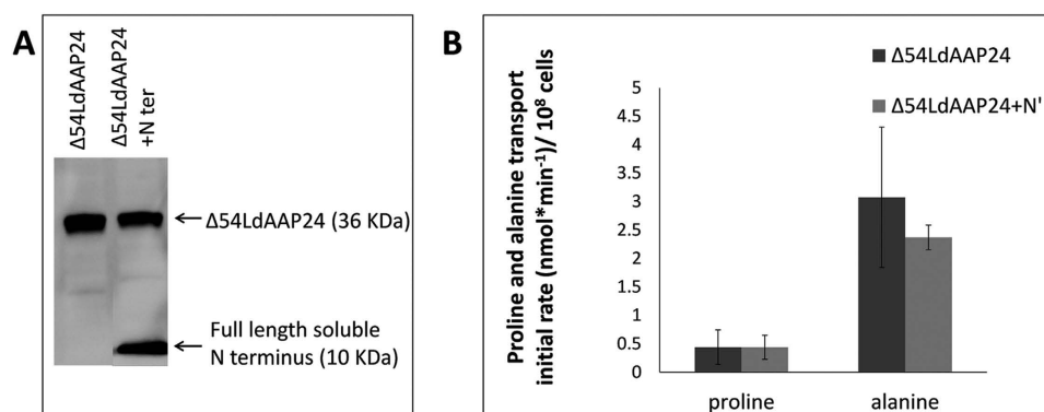
Figure 5. The soluble N-terminus cannot recover proline transport. (A) Western blot analysis of \Delta LdAAP24 ectopically co-expressing \Delta 54LdAAP24 (36kDa) and the full length N terminus (10kDa). (B) Initial transport rate (3 minutes) of 1 mM 3 H L-proline or 1 mM 3 H L-alanine were assayed in LdAAP24-null mutants ectopically expressing \Delta 54LdAAP24 (-N', dark grey) and LdAAP24-null mutants ectopically co-expressing \Delta 54LdAAP24 and the full length N terminus (+N', light grey). Transport was determined at pH 7 and 30°C. Values represent the mean of at least three independent repeats \pm SD.
