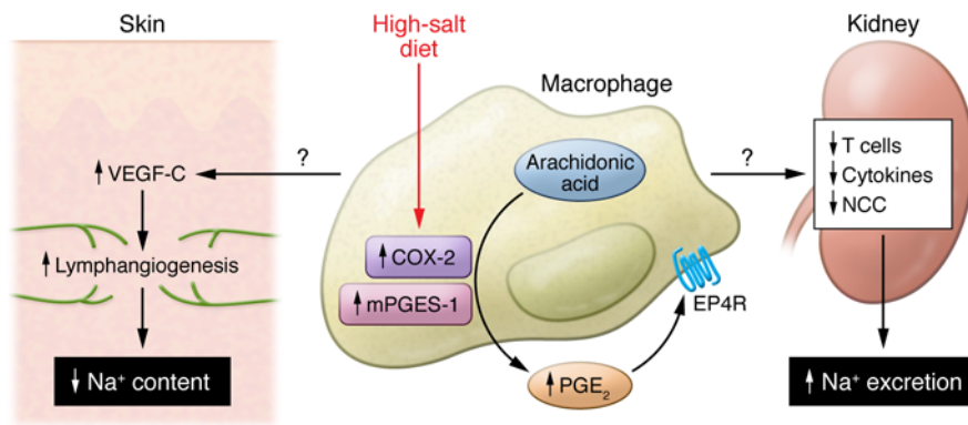
Figure 1. The COX-2/mPGES-1/EP4 receptor pathway in macrophages maintains sodium homeostasis by influencing salt secretion in the kidney and extrarenal sodium storage. In this issue, Zhang and colleagues demonstrate that a high-salt diet induces expression of COX-2, thereby enhancing PGE 2 production and autocrine EP4 receptor (EP4R) signaling. In mice lacking the COX-2/mPGES-1/EP4 receptor pathway in hematopoietic cells, extrarenal salt storage and sodium secretion by the kidney are dysfunctional, resulting in the development of hypertension.
