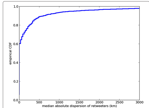
Figure 1 Empirical CDF of the median absolute deviation of retweeter locations of 4,004 forecasts generated by our model. With over 80% probability the retweeters are dispersed by less than 500 km.
