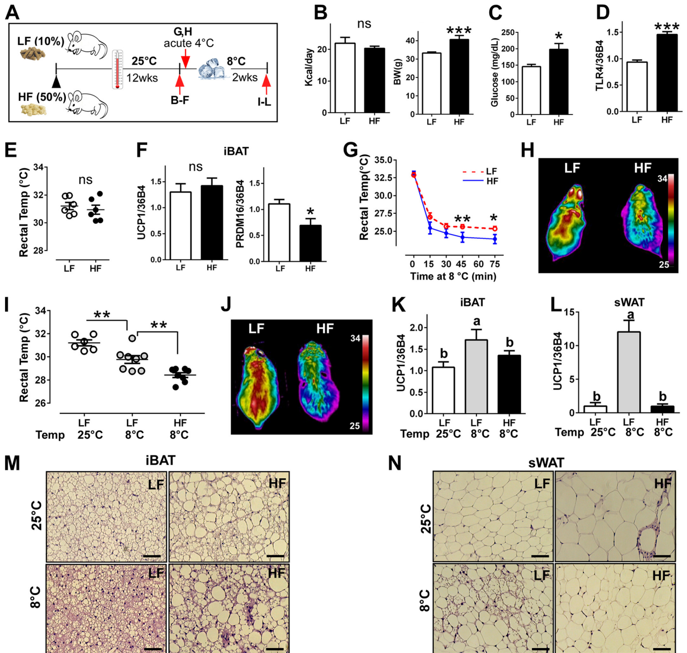
FIGURE 1. HF diet-induced TLR4 activation impaired adaptive thermogenesis. A , experimental scheme to determine the impacts of HF diet on adaptive thermogenesis. B–F , C57BL/6 mice were fed with HF versus LF diet for 12 weeks at 25 °C ( n = 8 per group). B , total calorie intake per day (left) and body weight difference (right). ns , not significant. C , fasting glucose levels. D , TLR4 mRNA expression by qPCR at the end of 12 weeks of the diet. E , core body temperature by rectal thermometer at the end of 12 weeks of diet. F , gene expression of UCP1 and PRDM16 by qPCR of iBAT. G and H , C57BL/6 mice were fed with the LF or HF diet for 12 weeks at 25 °C and exposed to 8 °C acutely. G , core body temperature upon cold exposure for 75 min ( n = 6 per group); red = LPS–, blue = LPS+. H , representative thermography captured by an IR camera ( n = 6–8 ). I–N , C57BL/6 mice were fed with HF versus LF diet for 12 weeks at 25 °C, then transferred to 8 °C for an additional 2 weeks ( n = 8 per group). I , core body temperature upon cold acclimation. J , representative thermography captured by an IR camera upon cold acclimation. K , UCP1 gene expression of iBAT after cold acclimation. L , UCP1 gene expression of sWAT after cold acclimation. M , representative images of H&E staining from iBAT (scale bar = 100 \mu\text{m} ). N , representative images of H&E staining from sWAT (scale bar = 100 \mu\text{m} ). All data are presented as the mean \pm S.E. *, p < 0.05 ; **, p < 0.01 ; ***, p < 0.001 by Student's t test. Values not sharing a common letter differ significantly ( p < 0.05 ) by one-way ANOVA.
