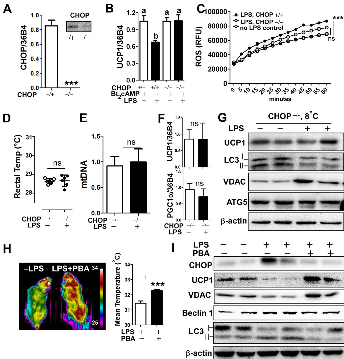
FIGURE 6. Inhibition of ER stress attenuated LPS-induced down-regulation of WAT browning and adaptive thermogenesis. A–C, primary adipocytes were prepared from EMSC of wild-type ( CHOP^{+/+} ) and CHOP deleted ( CHOP^{-/-} ) mice ( n = 4/\text{group} ). A, relative expression of mRNA of CHOP in CHOP^{+/+} versus CHOP^{-/-} adipocytes. B, relative expression of UCP1 with or without LPS pretreatment for 72 h followed by Bt 2 cAMP stimulation for 6 h. C, LPS-inducible ROS production in CHOP^{+/+} versus CHOP^{-/-} adipocytes ( n = 12 ). RFU, relative fluorescence units. ***, p < 0.001 by two-way ANOVA with repeated measure. D–G, CHOP^{-/-} mice received either saline or LPS injection every other day for 2 weeks at 8 °C ( n = 6 per group). D, core body temperature measured by rectal thermometer. E, mtDNA contents in sWAT after cold-acclimation. F, relative expression of UCP1 and PGC1 \alpha by qPCR of sWAT. G, Western blot analysis of UCP1, LC3I/II, VDAC, Atg5, and \beta -actin. H and I, C57BL/6 mice were injected with either saline, LPS alone, or LPS plus PBA (200 mg/kg/day) for 2 weeks at 8 °C ( n = 7 per each group). H, representative thermography captured by IR camera after cold acclimation (left). Mean surface body temperature was analyzed (right). I, Western blot analysis of CHOP, UCP1, LC3I/II, VDAC, Beclin1, and \beta -actin. All data are presented as the mean \pm S.E. ***, p < 0.001 by Student's t test; ns, non-significant. Values not sharing a common letter differ significantly ( p < 0.05 ) by one-way ANOVA.
