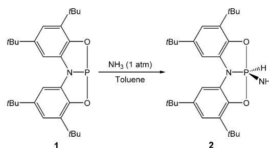
Scheme 2. The reaction of 1 with \text{NH}_3 to form 2 .
