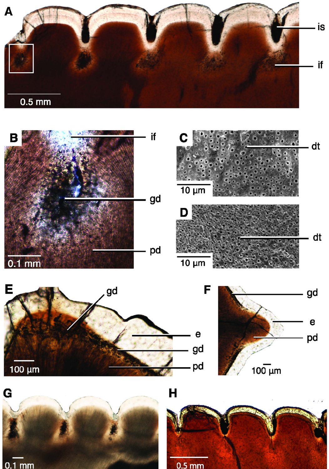
Figure 5. Microanatomy of unerupted cf. Gorgosaurus sp. teeth. (A) Distal carina of CMN 2225 showing the deep folds at the base of each interdigital sulcus. (B) Detail of interdigital fold from (A) showing absence of sclerotic dentine. (C) Dentine tubules in an erupted tooth (ROM 57981) showing peritubular dentine in each hollow tubule. (D) Dentine tubules in an unerupted tooth (CMN 2225) showing less peritubular dentine when compared to erupted tooth in (C). (E) Transverse section between two neighbouring denticles (CMN 2225), carina to the top. (F) Transverse section through a denticle showing absence of globular dentine in the denticle tip. Carina to the right. (G) Unerupted tooth of cf. Gorgosaurus libratus (RTMP 2012.012.0029), with interdigital folds. (H) Unerupted tooth of Allosaurus fragilis (UMNH.VP 23761), with interdigital folds. Abbreviations: dt, dentine tubule; e, enamel; gd, globular dentine; if, interdigital fold; is, interdigital sulcus; pd, primary dentine.
