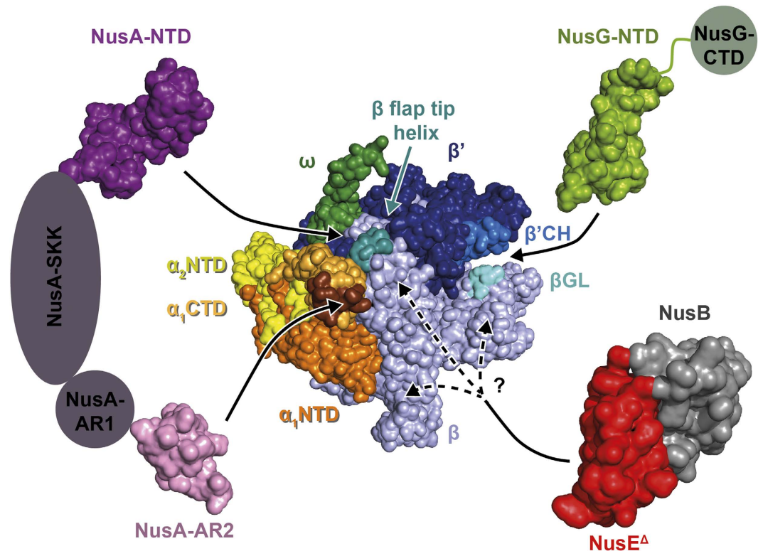
Figure 3. Nus factors binding sites on RNAP. RNAP is shown in surface representation with the NTD and CTD of \alpha subunit 1 in bright and pale orange, respectively, the NTD of \alpha subunit 2 in yellow, the \beta subunit in pale blue, the \beta' subunit in dark blue, the \omega subunit in dark green. Nus factor binding sites are highlighted (NusA-AR2 binding site on \alpha_1 CTD, brown; \beta GL, cyan; \beta flap tip helix, turquoise; \beta' CH, bright blue). Nus factors are displayed in surface representation with linker regions or domains not studied in this work being drawn schematically (NusG, bright green; NusA, purple; NusE A , red, NusB, grey). Black arrows indicate the binding site of each Nus factor or domain. NusE A interacts with the \beta subunit, but the exact binding site has not been identified yet. Protein Data Bank (PDB) codes: RNAP, 4KMU; NusA-NTD, 2KWP; NusA-AR2, 1WCN; NusB:NusE A , 3D3B; NusG-NTD, 2K06.
