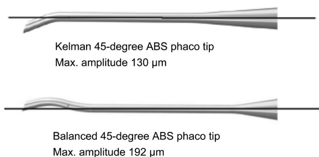
Figure 1 Configuration of 45-degree balanced and Kelman phaco tip and their maximum amplitudes.
