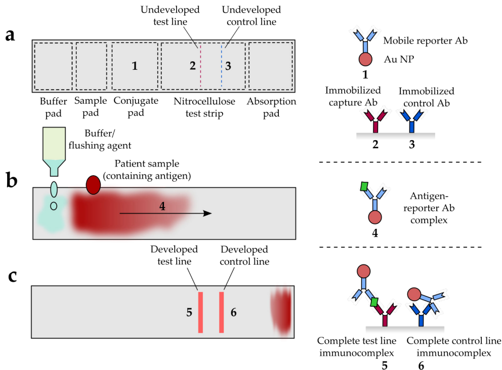
Figure 1. Standard configuration and mode of action for an immunochromatographic RDT. Note: Ab=antibody, Au NP=gold nanoparticle.
