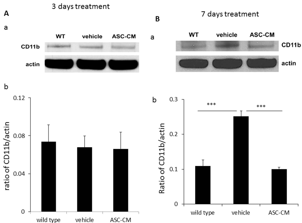
Figure 6. CD11b expression in spinal cords of symptomatic SOD1 G93A mice after 3 days or 7 days of ASC-CM treatment. SOD1 G93A mice were given 3 days or 7 days of ASC-CM treatment or vehicle upon disease onset. Spinal cords were processed Western blot as described in Experimental Procedures. Unchanged actin levels in all groups were used as internal loading controls. (A) (a) The representative immunoblots and (b) band densities that were measured showed no change in spinal cord CD11b expression after 7 days of ASC-CM treatment. (B) (a) The representative immunoblots and (b) band quantitation demonstrated a decrease in spinal cord CD11b expression after 7 days of ASC-CM treatment as compared to vehicle. n = 3 , *** p < 0.005 .
