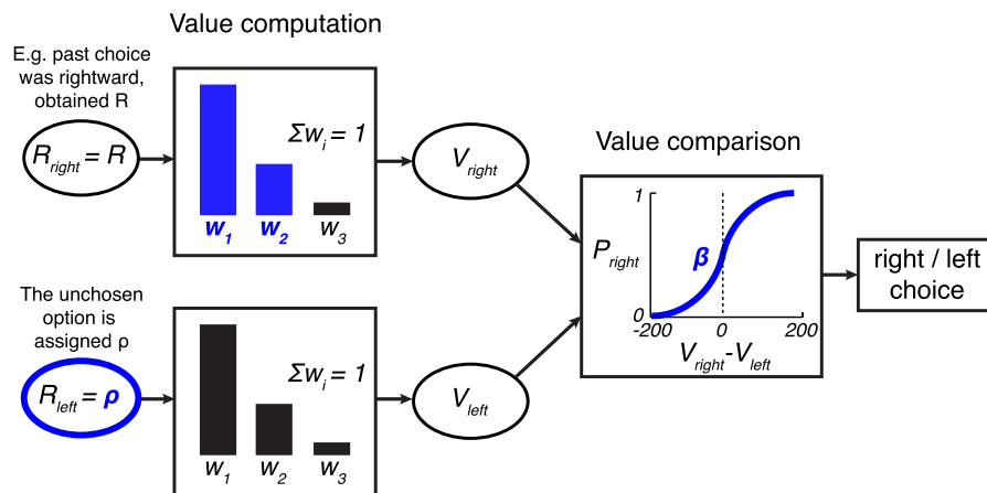
Figure 3. The model. In the model, an option is assigned the reward obtained from the according choice, of magnitude R . The unchosen option is assigned a value of \rho , a free parameter. The past three rewards obtained for each option r_i are linearly weighted to obtain the value of an option, V = \sum_{i=1}^3 w_i r_i . The weights w_1 and w_2 are free parameters; w_3 = 1 - w_1 - w_2 . The values V_{\text{right}} and V_{\text{left}} are then compared using a sigmoid choice function \Psi(V_{\text{right}} - V_{\text{left}}) whose steepness is parametrized by \beta . This results in the model's output: the probability of choosing the rightward option P_{\text{right}} in each trial. The model's free parameters are highlighted in blue.
