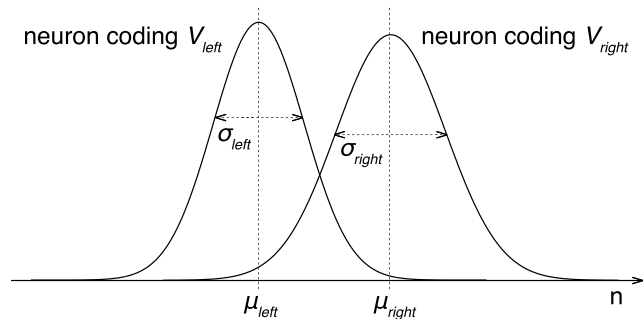
Figure 11. Representation of option values by spiking neurons.
