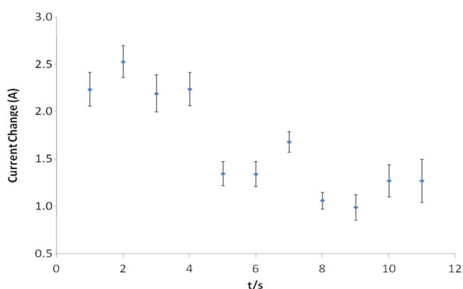
Figure 6. Moving average of the current change observed for a typical response obtained (Figure 5A) for wild type MPI cells exposed to LPS.
