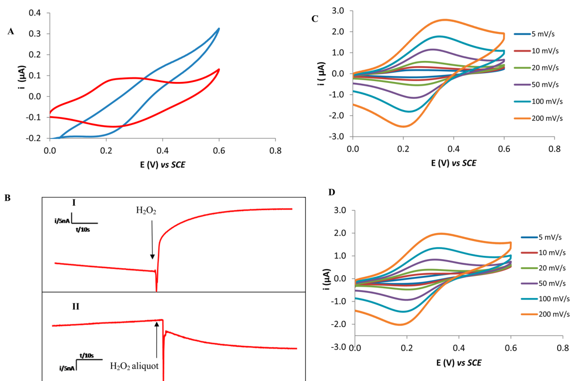
Figure 1. (A) Typical cyclic voltammograms obtained in PBS (red) and 100 mM H 2 O 2 (blue) at an ITO-SWCNTs-Osbpy electrode at a scan rate of 5 mV s -1 . (B) Typical fixed potential amperograms obtained for addition of 1 mM aliquots of H 2 O 2 to PBS using an ITO-SWCNT-Osbpy electrode poised 400 mV (I) to establish the presence of oxidative processes and at 150 mV (II) to investigate the reductive processes. (C, D) Typical cyclic voltammograms obtained for (C) PBS and in (D) 100 mM H 2 O 2 solutions at ITO-SWCNT-Osbpy electrode at 5, 10, 20, 50, 100, and 200 mV s -1 .
