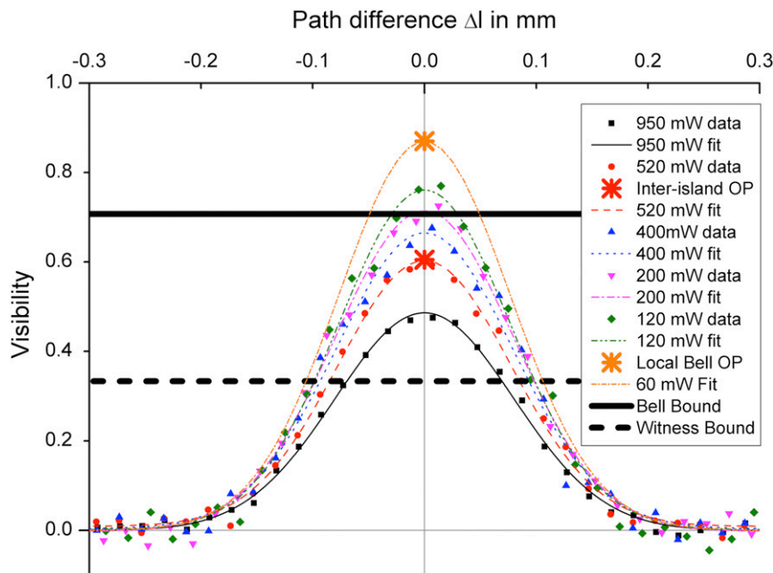
Fig. 2. Plot of the entanglement-swapping visibility versus path-length difference for different pump powers locally measured on La Palma. The abscissa represents the relative optical path-length difference \Delta l in mm between photon “1” and “2” in the BSM and the ordinate represents the entanglement-swapping visibility. Black squares, red dots, blue triangles, purple upside-down triangles, and green diamonds indicate the data points of the visibilities at 950-, 520-, 400-, 200-, and 120-mW average pump power, respectively. The entanglement-witness bound and the bound for the violation of a CHSH-type Bell inequality are represented by a black dashed and a black solid line at visibilities of 1/3 and 1/\sqrt{2} , respectively. The operating point (OP) for the local test of the CHSH inequality was chosen at a pump power of 60 mW and zero delay (orange asterisk). At this set point a visibility of 0.87 was achieved. For the entanglement-swapping experiment via the 143-km and -32 -dB free-space link we tuned the setup to a visibility of 0.6 at 520-mW average pump power (red asterisk) and again perfect overlap at zero delay.
