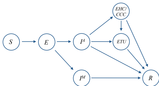
Fig. 1. Model structure. Individuals start off susceptible to infection (S). Upon infection with Ebola they enter an incubation period (E), then at symptom onset they become infectious; these individuals either eventually become ascertained ( I^A ) or do not ( I^M ). Individuals who are ascertained initially seek health care in EHCs/CCCs (or ETUs if these are full); if no beds are available, they remain infectious in the community until the infection is resolved (R), i.e., they have recovered, or are dead and buried. Patients in EHC/CCCs are transferred to ETUs once they have been tested for Ebola, which takes an average of 2 d. Patients remain in ETUs until the infection is resolved. We assume the latent period is 9.4 d, the average time from onset to EHC/CCC attendance declines from an initial value of 4.6 d ( SI Appendix, Fig. S1 ), and individuals who do not seek treatment are infectious for 10.9 d on average (details in SI Appendix ).
