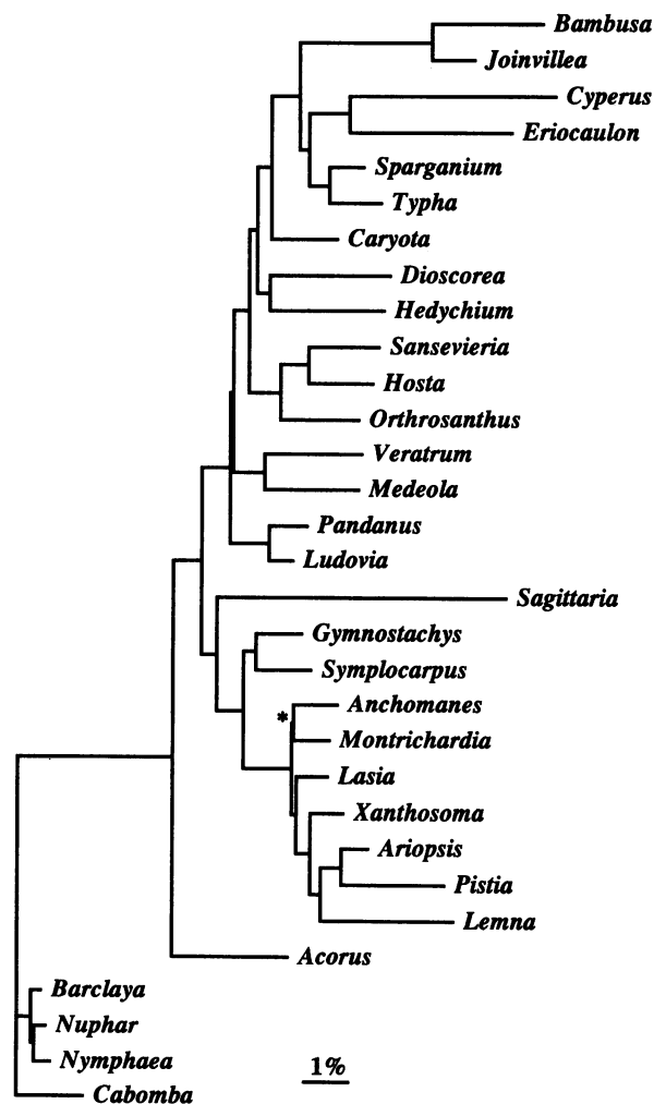
FIG. 1. The maximum likelihood topology with the largest (least negative) log-likelihood score of 17 replicated maximum likelihood analyses of rbcL sequences from 27 species of monocotyledons and 4 outgroup species of Nymphaeanae (water lilies). Branch lengths correspond to evolutionary distances. Scale bar indicates 1% sequence divergence. All branches are significantly positive at the P = 0.05 level with the exception of that marked with an asterisk.
