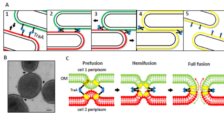
Fig. 2. Model for outer membrane exchange (OME) in myxobacteria. A) 1) TraA-TraA recognition occurs between neighboring cells. Green and red symbolize different fluorescent markers in the OM. 2) Cells are brought into close proximity upon recognition and motility. 3) 'Prefusion junctions' form and cells continue to move. 4) Motility helps trigger fusion to facilitate OM exchange. 5) Cells separate after OME. B) TraAB overexpression leads to cell-cell 'prefusion junctions' (arrows) as seen by cryo-electron microscopy. Cross-section shows center cell interacting with three neighboring cells. Bar, 100 nm [85]. C) Schematic model of OM fusion dynamics (based on eukaryotic models) during OME. Upon TraA-TraA interaction, the OMs of two aligned cells come into close contact and form a prefusion junction. The outer leaflets of the two OMs then fuse creating a hemifusion complex. Subsequently, full fusion of the OM (both outer and inner leaflets) is presumed to occur, though soluble periplasmic proteins have not been found to transfer. Dashed arrows indicate lateral diffusion of OM components between cells.
