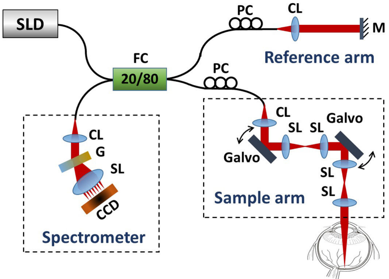
Figure 1. Schematic of the 147 kHz spectral-domain OCT imaging system. CCD, line scan camera; CL, collimating lens; FC, fiber coupler; G, grating; Galvo, 1D galvanometer; M, mirror; PC, polarization controller; SL, scan lens.
