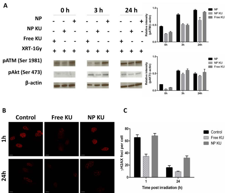
Figure 4. Effect of KU55933 formulations and radiation on phosphorylation of ATM, Akt and H2AX. H460 cells were pretreated with 10 \mu M KU or NP KU (containing 10 \mu M KU) for 3 h and subsequently irradiated (1 Gy). (A) Cell lysates were collected at indicated time points for western blot. The western blot band intensity was quantified after normalized to \beta -actin based on three independent experiments. (B) Cells were fixed at indicated time points for immunofluorescence of \gamma H2AX. (C) Average numbers of \gamma H2AX foci per cell were presented.
