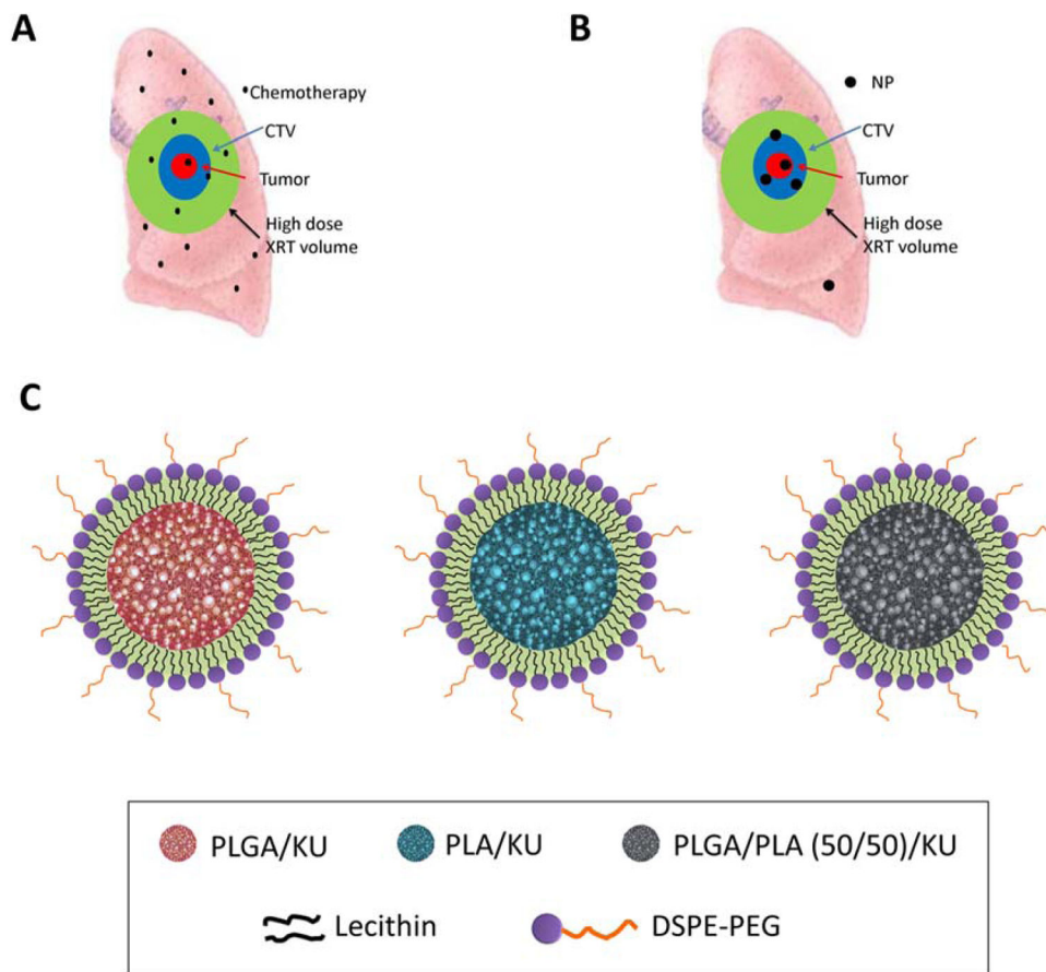
Figure 1. Diagram of chemoradiotherapy for lung cancer. The red area is the gross tumor. Blue area is CTV (clinical target volume), which is the area of lung that should receive high dose radiotherapy and radiosensitizer. Green area indicates the area of lung tissue that receives high dose radiotherapy (XRT) because of motion, entrance and exit radiotherapy dose. In conventional treatment (A) with small molecule chemotherapeutics such as KU55933, the green area receives both high dose radiotherapy and radiosensitizers. In contrast, NP therapeutics (B) concentrate in tumors and minimize the area of normal lung that receives both radiotherapy and radiosensitizer/chemotherapy. (C) Cartoon of NP KU55933 with different lipid polymers.
