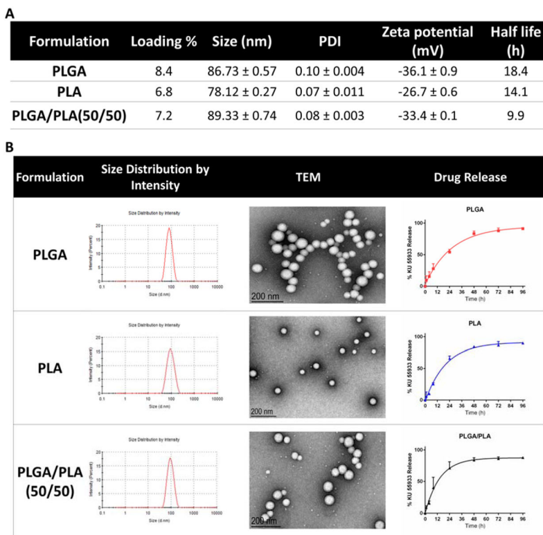
Figure 2. Characterization of NP KU5933 with different lipid polymers. (A) Comparison of different lipid polymer formulations of NP KU5933 in drug loading efficacy, size, zeta potential and half-life. (B) Nanoparticle size distribution, TEM image and release profile of NP KU5933. Values are represented as mean ± standard error (n=3).
