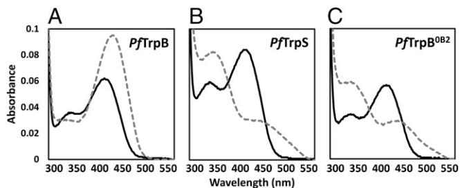
Fig. 2. UV-vis absorption spectra of native and engineered PflTrpB . (A) The PLP absorption spectrum of PflTrpB (black) has a \lambda_{\text{max}} = 412 nm, characteristic of E(Ain). Addition of 20 mM L-serine causes a red-shift to 428 nm (gray), consistent with E(Aex 1 ) formation. (B) Addition of L-serine to PflTrpS causes a shift in \lambda_{\text{max}} to 350 nm, which is attributed to the E(A-A). A residual peak at 428 nm indicates population of E(Aex 1 ). (C) Like PflTrpS , addition of 20 mM L-serine to PflTrpB OB2 shows \lambda_{\text{max}} = 350 nm as well as contributions from E(Aex 1 ). All spectra were collected with 20 \mu\text{M} of enzyme. See Materials and Methods for details.
