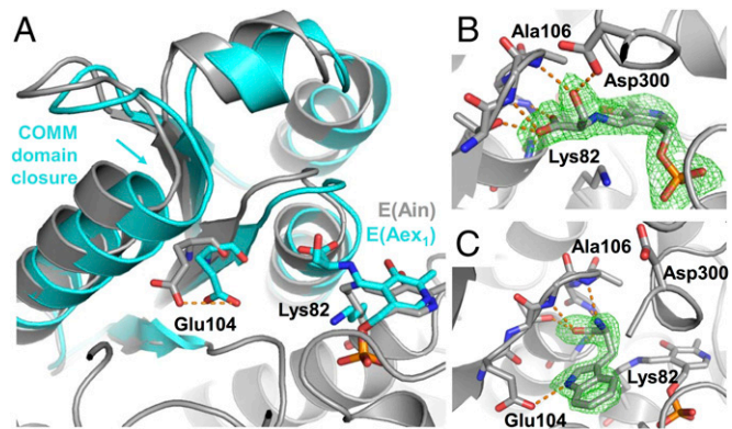
Fig. 3. Structural transitions upon ligand binding in PflTrpB . (A) Superimposition of PflTrpB -E(Ain) and PflTrpB -E(Aex 1 ) in gray and cyan, respectively. Overlay shows the 2.1-Å displacement of the COMM domain upon E(Aex 1 ) formation. This closure moves the side chain of Glu104 by 3.7 Å, toward its catalytic orientation (orange dashes). (B) Structure of Ser-bound PflTrpB with a F_0 - F_c map of E(Aex 1 ) contoured at 3.0 \sigma (green). (C) Structure of L-tryptophan-bound PflTrpB with F_0 - F_c map of Trp ligand contoured at 3.0 \sigma .
