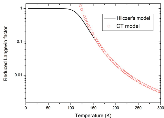
Figure 2. Temperature dependence behaviors of the Langevin reduction factor \gamma predicted by the continuum model 13 and the CT model. 18 Both curves are based on the parameters that fit the experimental \gamma – T data of ref 7.
