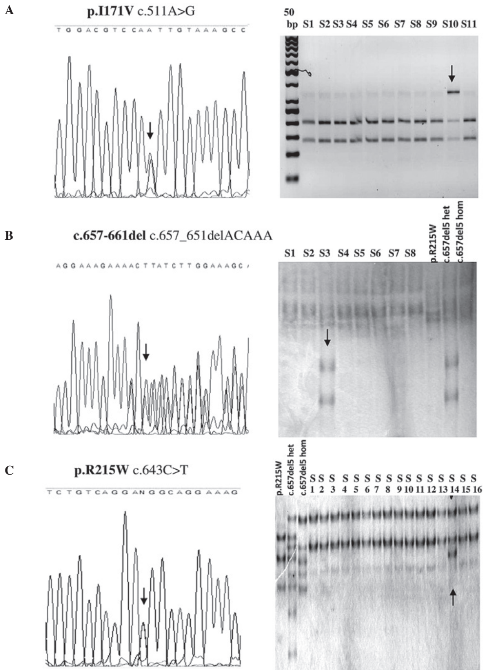
Figure 2. (A) Sequencing results and RFLP analysis (using MunI restriction enzyme) corresponding to the p. I171V variant. Sequencing and SSCP analysis of the variants (B) c.657del5 and (C) p.R215W. The variants are indicated by an arrow. RFLP, restriction fragment length polymorphism; SSCP, single-strand conformation polymorphism; S, sample; p.R215W, reference sequence for heterozygous p.R215W substitution; c.657del5 het, reference sequence for heterozygous c.657del5 mutation; c.657del5 hom, reference sequence for homozygous c.657del5 mutation.
