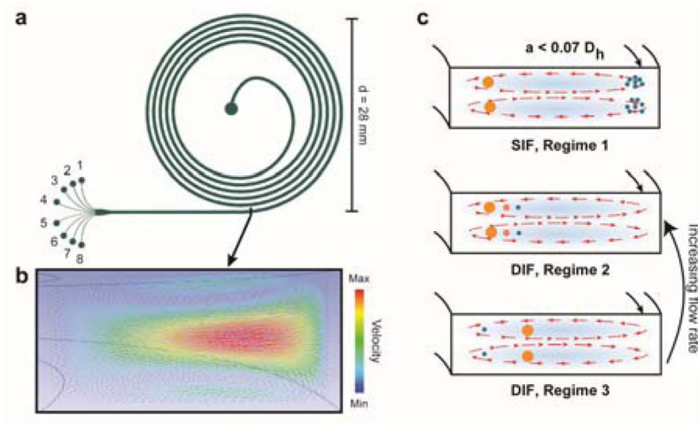
Figure 2. Schematics depicting the design and working principle of the sorting device a) Schematic of the device geometry, inlet and eight outlets. b) Numerical simulation showing the secondary flow field at the outlet. c) Schematic showing different focusing regimes in inertial microfluidics. In SIF, regime 1, only the particles of interest are focused while the others are entrained in the vortices. In DIF, regime 2, the particles are focused in descending order of size from the inner wall. In DIF, regime 3, the smaller particles are focused near the inner wall, while the larger ones are focused in the center. Regime 3 transitions to regime 2 with increasing flow rate.
